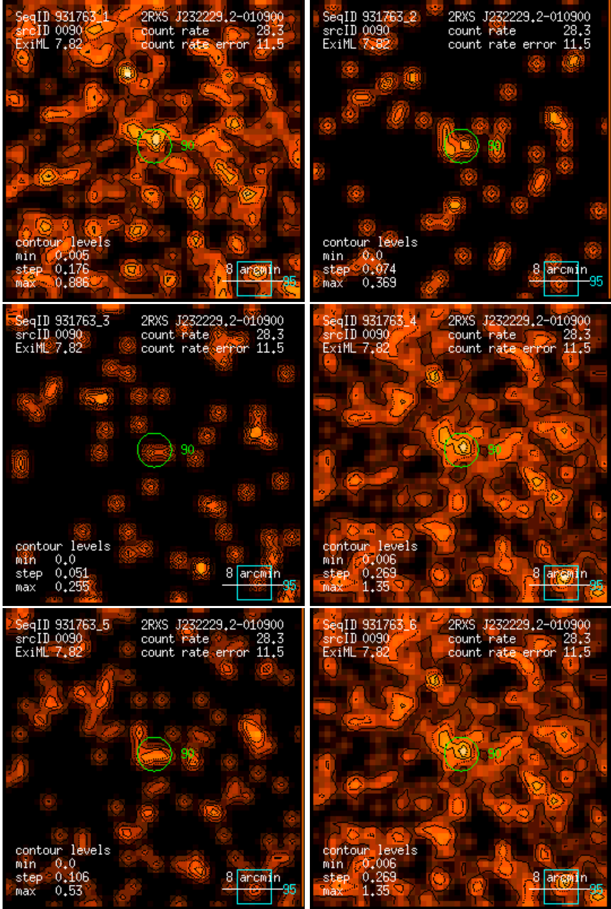
Figure 90: RASS 931763: detection 0090: band rate images, Gaussian filter: (1) PSPC channels 11 – 41, (2) 52 – 90, (3) 91 – 201, (4) 11 – 235, (5) 52 – 201, (6) 11 – 201. Broad band rates in counts/ks. Band rate contour levels in counts/ks/arcmin 2 .
