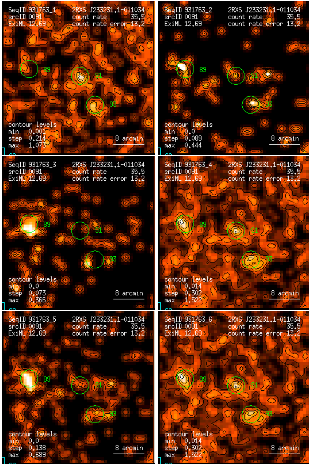
Figure 91: RASS 931763: detection 0091: band rate images, Gaussian filter: (1) PSPC channels 11 – 41, (2) 52 – 90, (3) 91 – 201, (4) 11 – 235, (5) 52 – 201, (6) 11 – 201. Broad band rates in counts/ks. Band rate contour levels in counts/ks/arcmin 2 .
