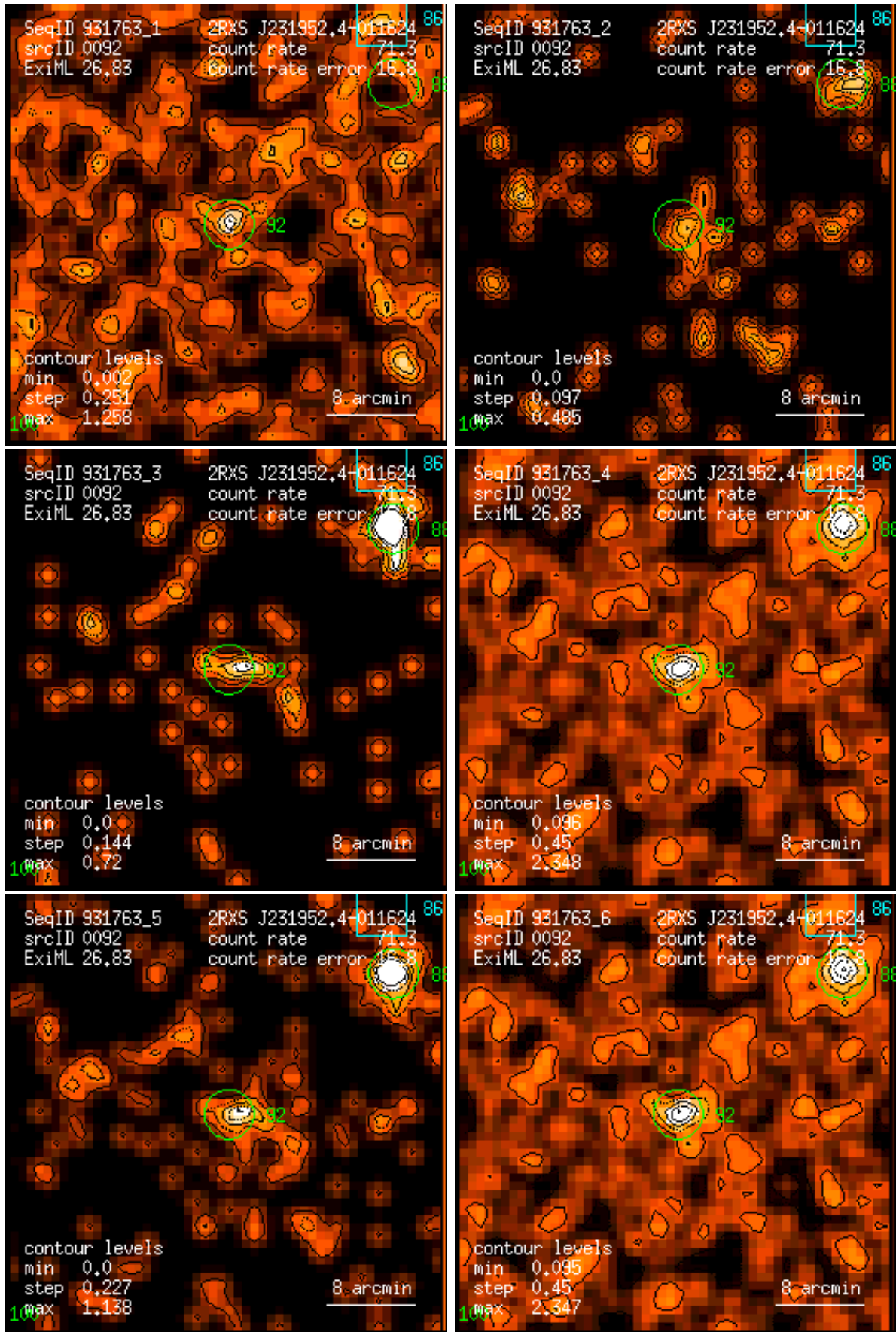
Figure 92: RASS 931763: detection 0092: band rate images, Gaussian filter: (1) PSPC channels 11 – 41, (2) 52 – 90, (3) 91 – 201, (4) 11 – 235, (5) 52 – 201, (6) 11 – 201. Broad band rates in counts/ks. Band rate contour levels in counts/ks/arcmin 2 .
