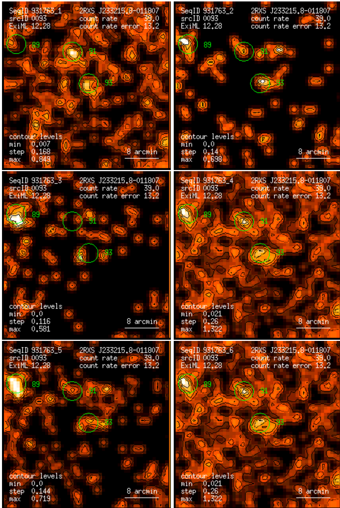
Figure 93: RASS 931763: detection 0093: band rate images, Gaussian filter: (1) PSPC channels 11 – 41, (2) 52 – 90, (3) 91 – 201, (4) 11 – 235, (5) 52 – 201, (6) 11 – 201. Broad band rates in counts/ks. Band rate contour levels in counts/ks/arcmin 2 .
