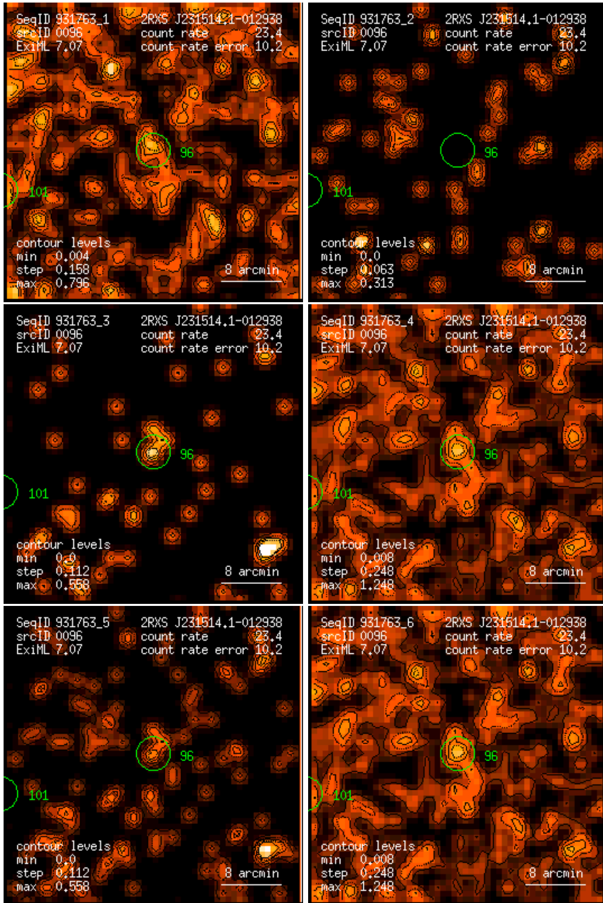
Figure 96: RASS 931763: detection 0096: band rate images, Gaussian filter: (1) PSPC channels 11 – 41, (2) 52 – 90, (3) 91 – 201, (4) 11 – 235, (5) 52 – 201, (6) 11 – 201. Broad band rates in counts/ks. Band rate contour levels in counts/ks/arcmin 2 .
