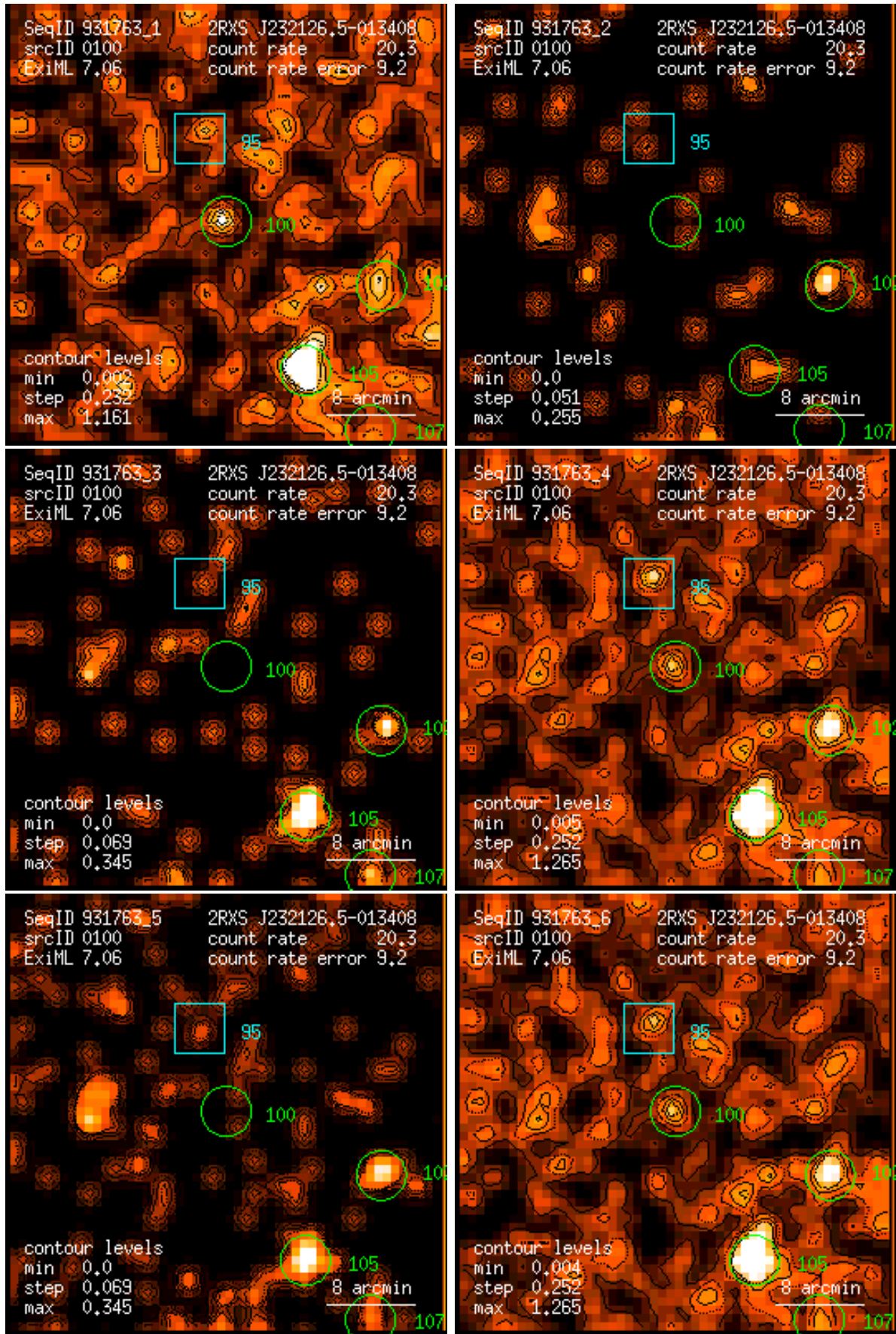
Figure 100: RASS 931763: detection 0100: band rate images, Gaussian filter: (1) PSPC channels 11 – 41, (2) 52 – 90, (3) 91 – 201, (4) 11 – 235, (5) 52 – 201, (6) 11 – 201. Broad band rates in counts/ks. Band rate contour levels in counts/ks/arcmin 2 .
