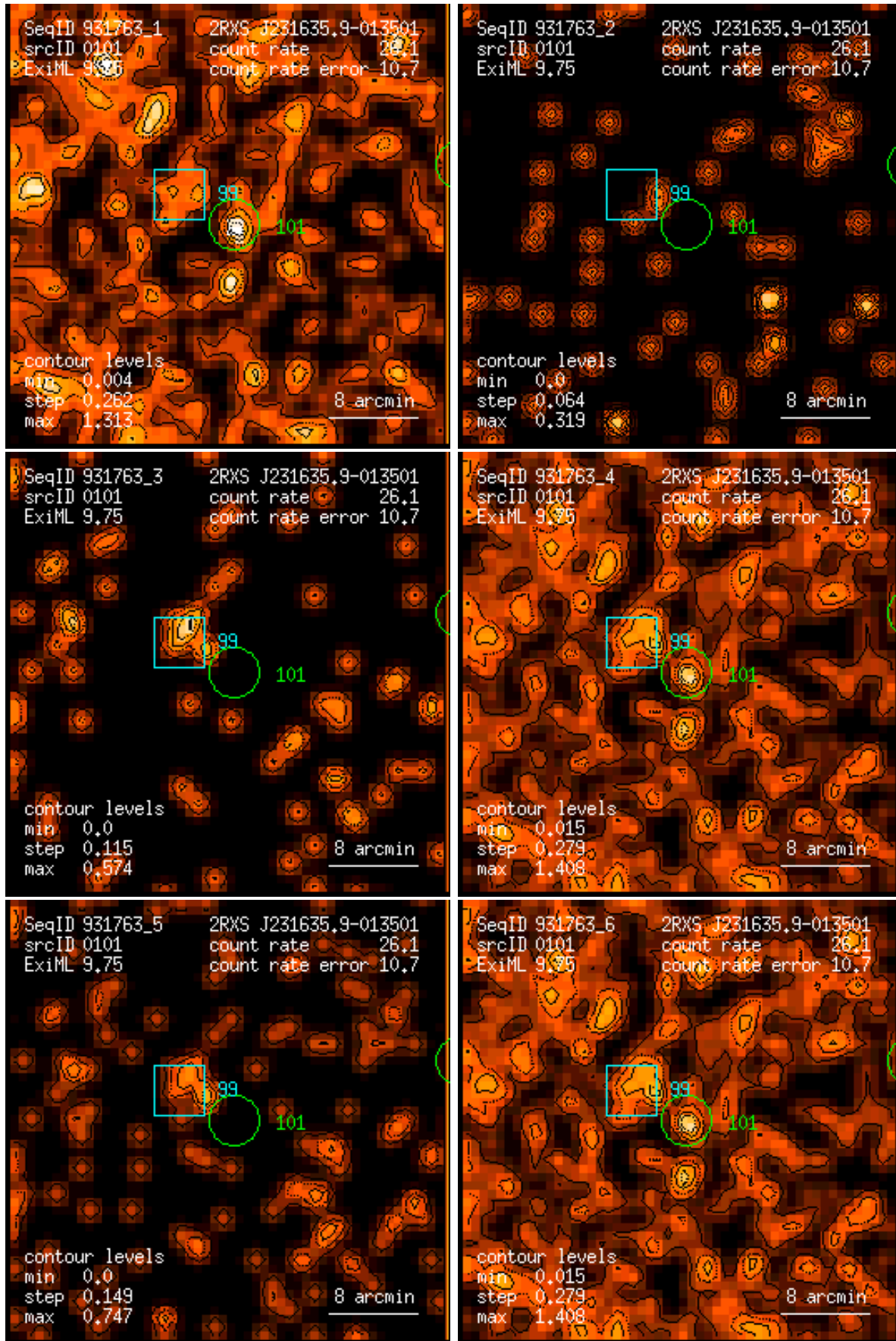
Figure 101: RASS 931763: detection 0101: band rate images, Gaussian filter: (1) PSPC channels 11 – 41, (2) 52 – 90, (3) 91 – 201, (4) 11 – 235, (5) 52 – 201, (6) 11 – 201. Broad band rates in counts/ks. Band rate contour levels in counts/ks/arcmin 2 .
