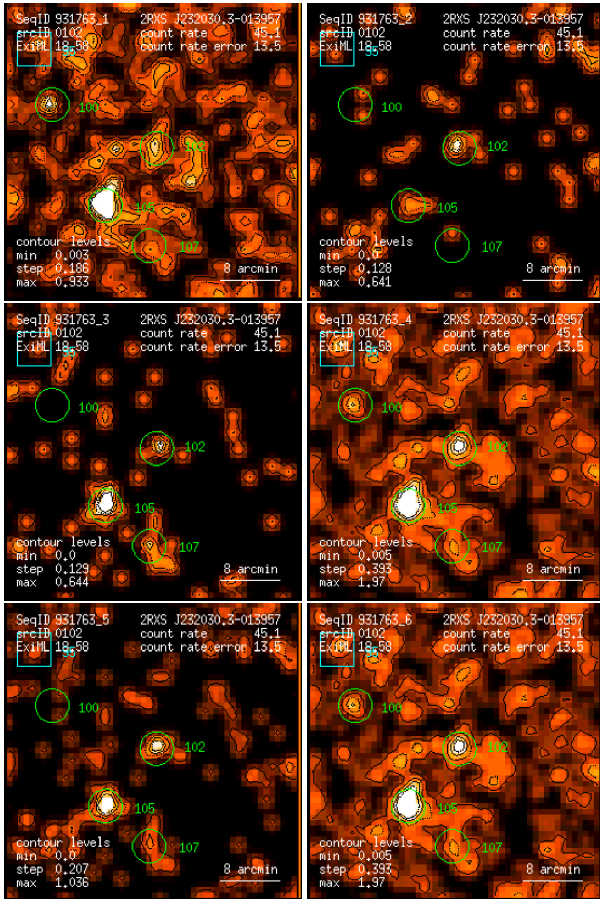
Figure 102: RASS 931763: detection 0102: band rate images, Gaussian filter: (1) PSPC channels 11 – 41, (2) 52 – 90, (3) 91 – 201, (4) 11 – 235, (5) 52 – 201, (6) 11 – 201. Broad band rates in counts/ks. Band rate contour levels in counts/ks/arcmin 2 .
