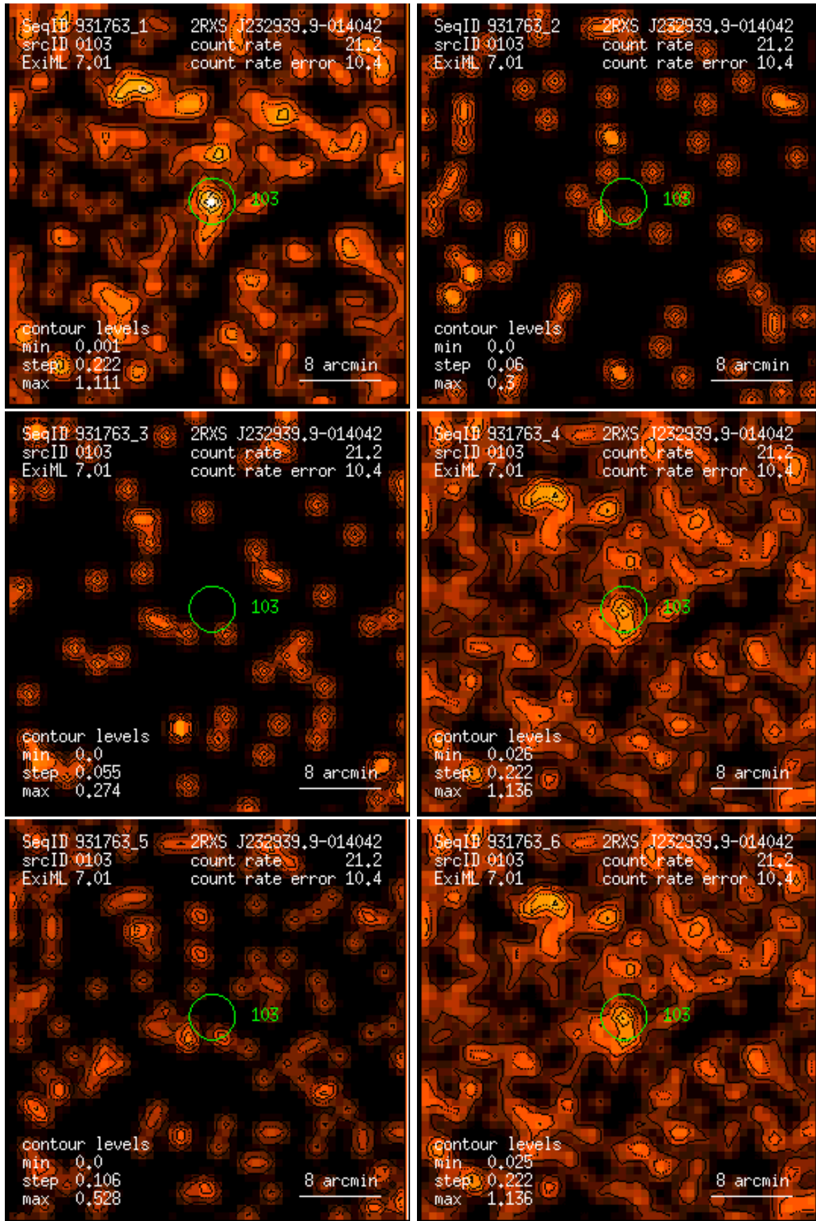
Figure 103: RASS 931763: detection 0103: band rate images, Gaussian filter: (1) PSPC channels 11 – 41, (2) 52 – 90, (3) 91 – 201, (4) 11 – 235, (5) 52 – 201, (6) 11 – 201. Broad band rates in counts/ks. Band rate contour levels in counts/ks/arcmin 2 .
