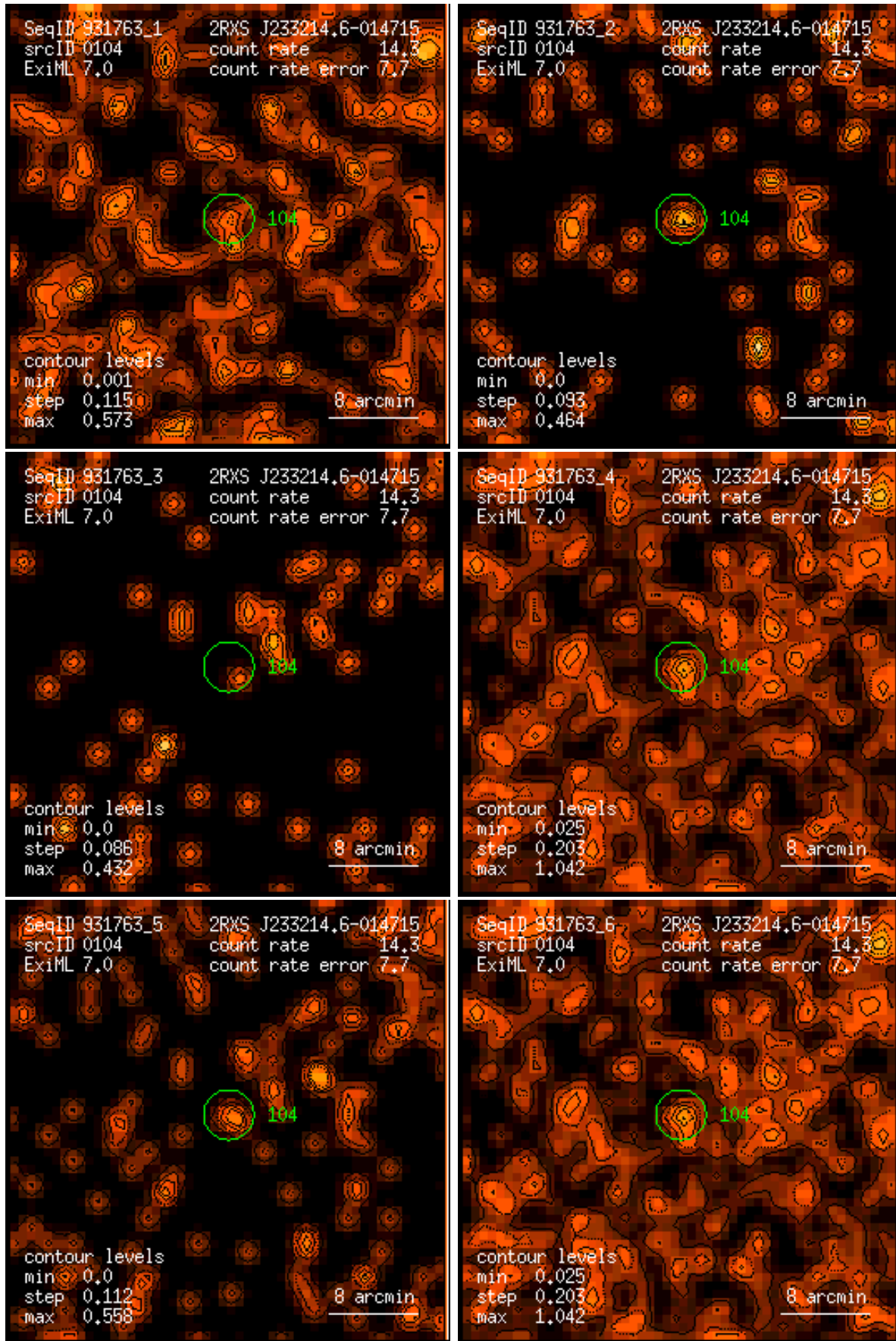
Figure 104: RASS 931763: detection 0104: band rate images, Gaussian filter: (1) PSPC channels 11 – 41, (2) 52 – 90, (3) 91 – 201, (4) 11 – 235, (5) 52 – 201, (6) 11 – 201. Broad band rates in counts/ks. Band rate contour levels in counts/ks/arcmin 2 .
