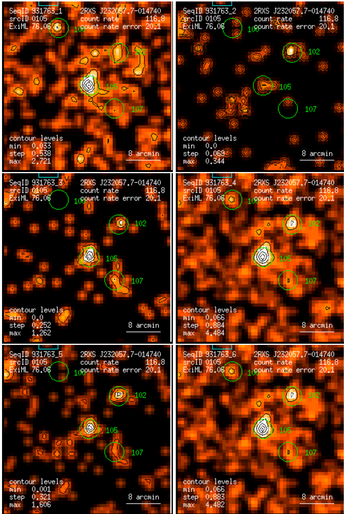
Figure 105: RASS 931763: detection 0105: band rate images, Gaussian filter: (1) PSPC channels 11 – 41, (2) 52 – 90, (3) 91 – 201, (4) 11 – 235, (5) 52 – 201, (6) 11 – 201. Broad band rates in counts/ks. Band rate contour levels in counts/ks/arcmin 2 .
