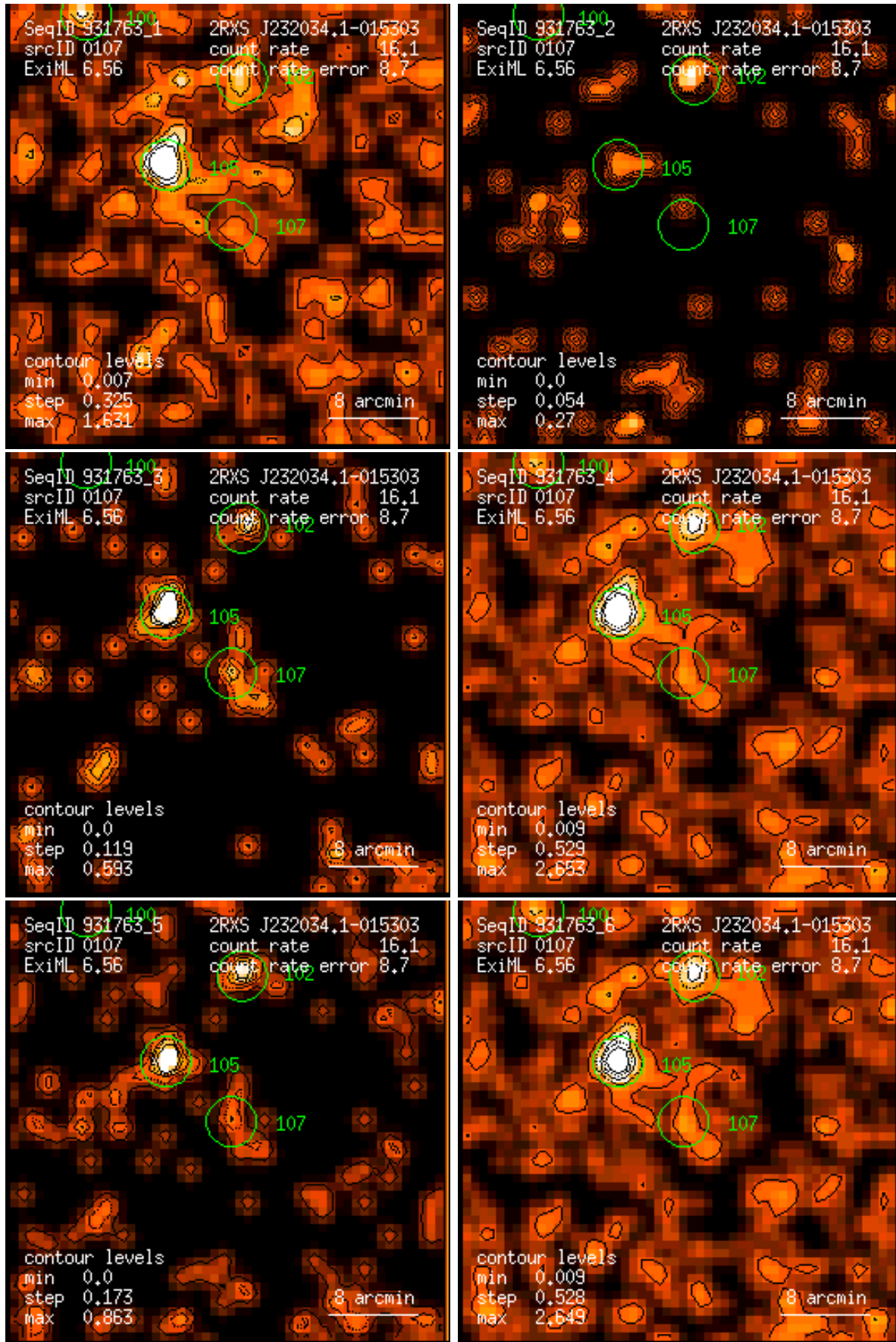
Figure 107: RASS 931763: detection 0107: band rate images, Gaussian filter: (1) PSPC channels 11 – 41, (2) 52 – 90, (3) 91 – 201, (4) 11 – 235, (5) 52 – 201, (6) 11 – 201. Broad band rates in counts/ks. Band rate contour levels in counts/ks/arcmin 2 .
