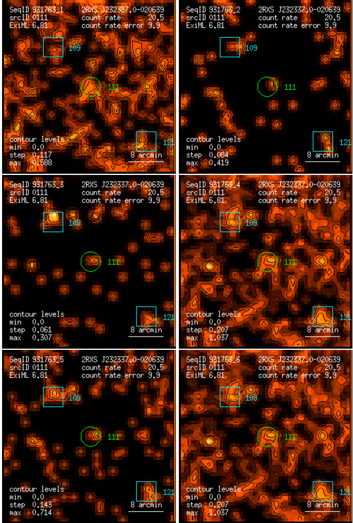
Figure 111: RASS 931763: detection 0111: band rate images, Gaussian filter: (1) PSPC channels 11 – 41, (2) 52 – 90, (3) 91 – 201, (4) 11 – 235, (5) 52 – 201, (6) 11 – 201. Broad band rates in counts/ks. Band rate contour levels in counts/ks/arcmin 2 .
