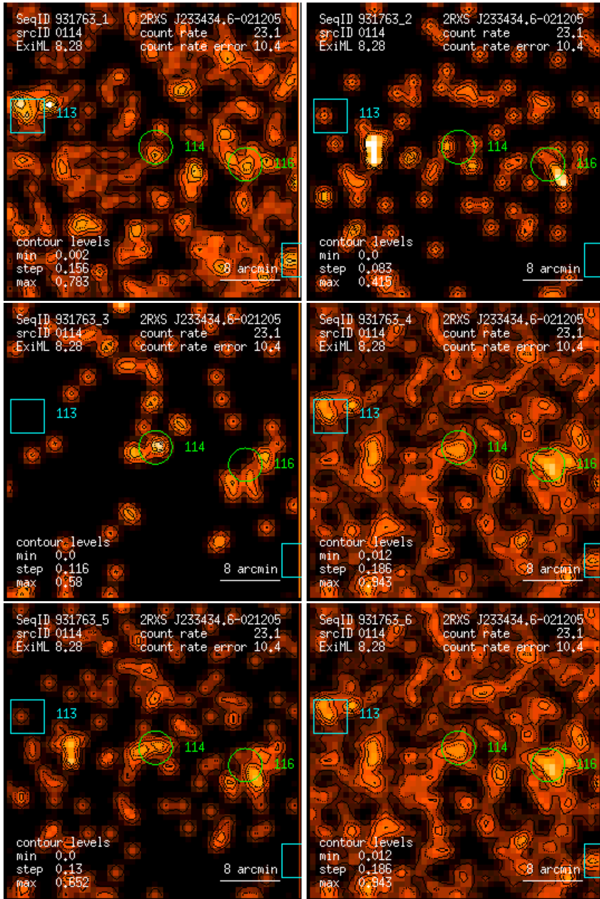
Figure 114: RASS 931763: detection 0114: band rate images, Gaussian filter: (1) PSPC channels 11 – 41, (2) 52 – 90, (3) 91 – 201, (4) 11 – 235, (5) 52 – 201, (6) 11 – 201. Broad band rates in counts/ks. Band rate contour levels in counts/ks/arcmin 2 .
