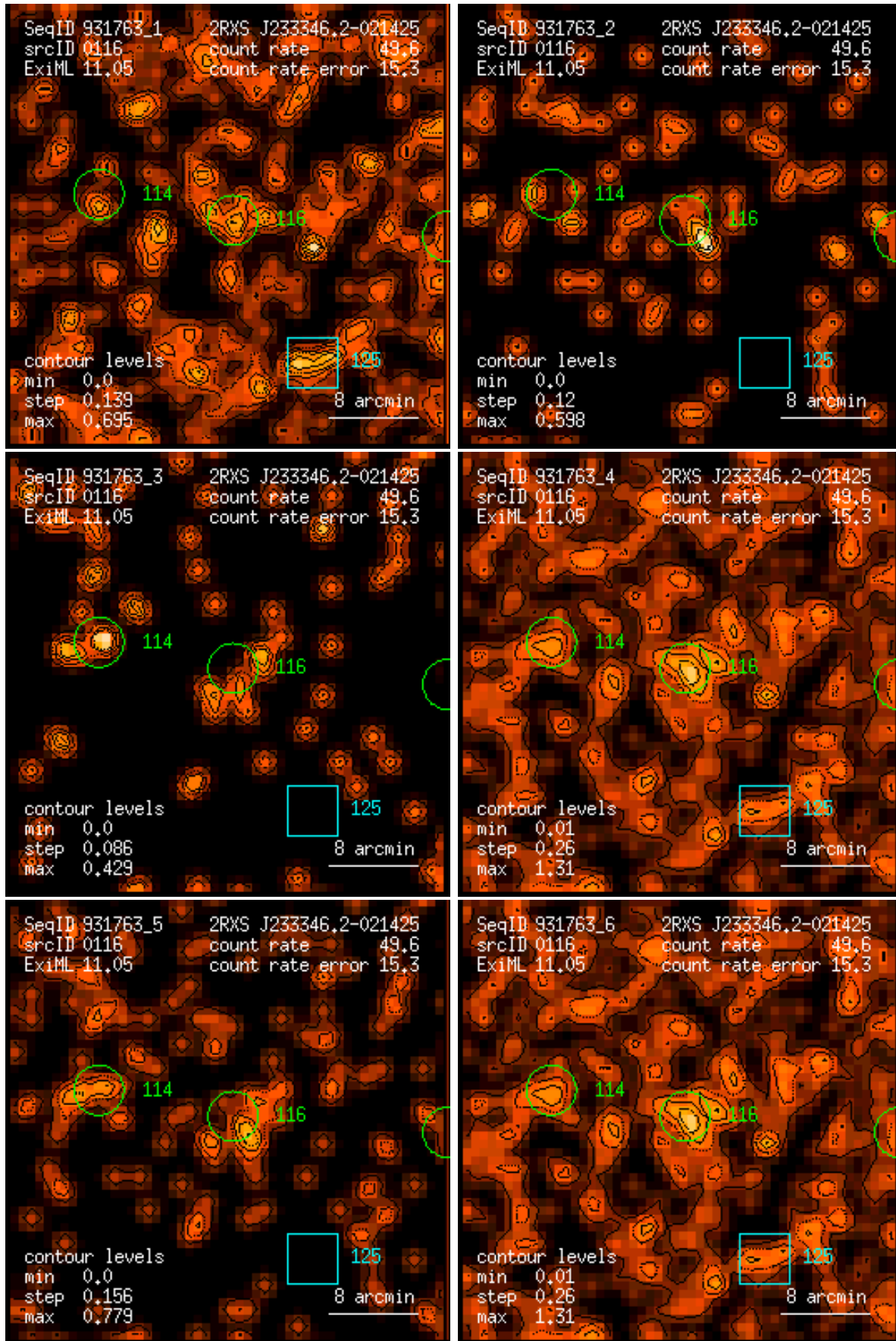
Figure 116: RASS 931763: detection 0116: band rate images, Gaussian filter: (1) PSPC channels 11 – 41, (2) 52 – 90, (3) 91 – 201, (4) 11 – 235, (5) 52 – 201, (6) 11 – 201. Broad band rates in counts/ks. Band rate contour levels in counts/ks/arcmin 2 .
