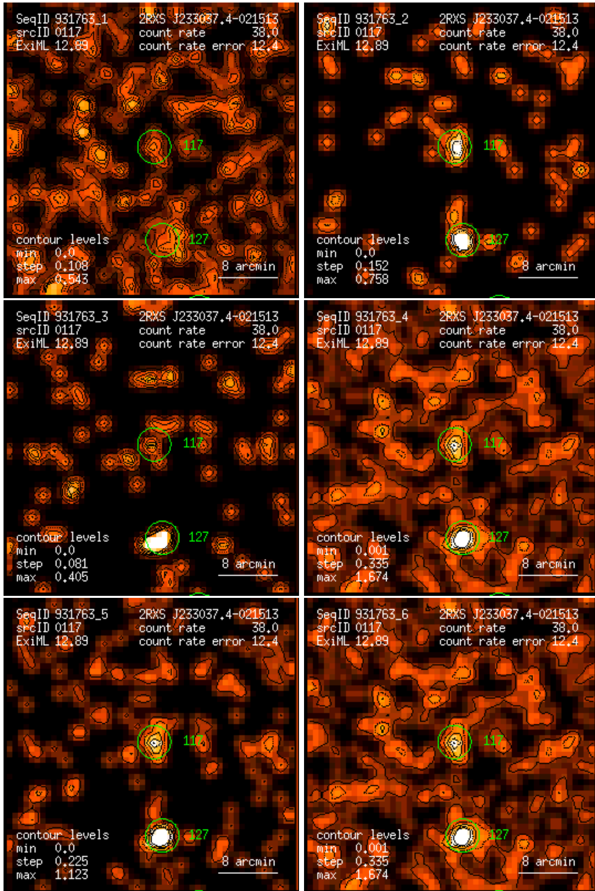
Figure 117: RASS 931763: detection 0117: band rate images, Gaussian filter: (1) PSPC channels 11 – 41, (2) 52 – 90, (3) 91 – 201, (4) 11 – 235, (5) 52 – 201, (6) 11 – 201. Broad band rates in counts/ks. Band rate contour levels in counts/ks/arcmin 2 .
