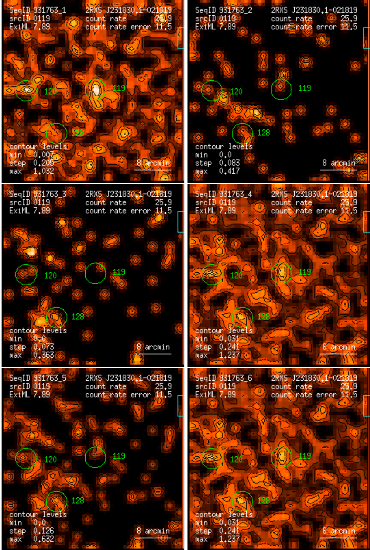
Figure 119: RASS 931763: detection 0119: band rate images, Gaussian filter: (1) PSPC channels 11 – 41, (2) 52 – 90, (3) 91 – 201, (4) 11 – 235, (5) 52 – 201, (6) 11 – 201. Broad band rates in counts/ks. Band rate contour levels in counts/ks/arcmin 2 .
