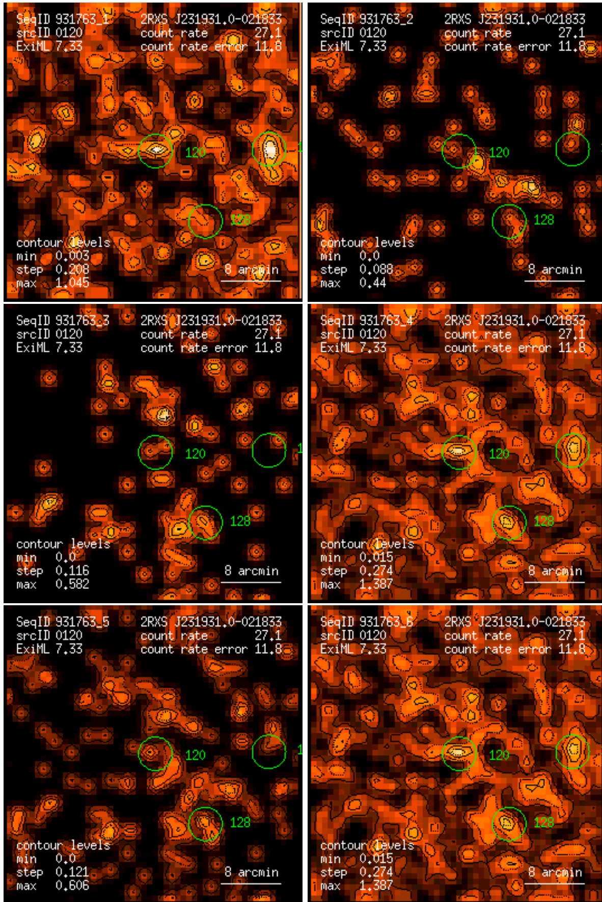
Figure 120: RASS 931763: detection 0120: band rate images, Gaussian filter: (1) PSPC channels 11 – 41, (2) 52 – 90, (3) 91 – 201, (4) 11 – 235, (5) 52 – 201, (6) 11 – 201. Broad band rates in counts/ks. Band rate contour levels in counts/ks/arcmin 2 .
