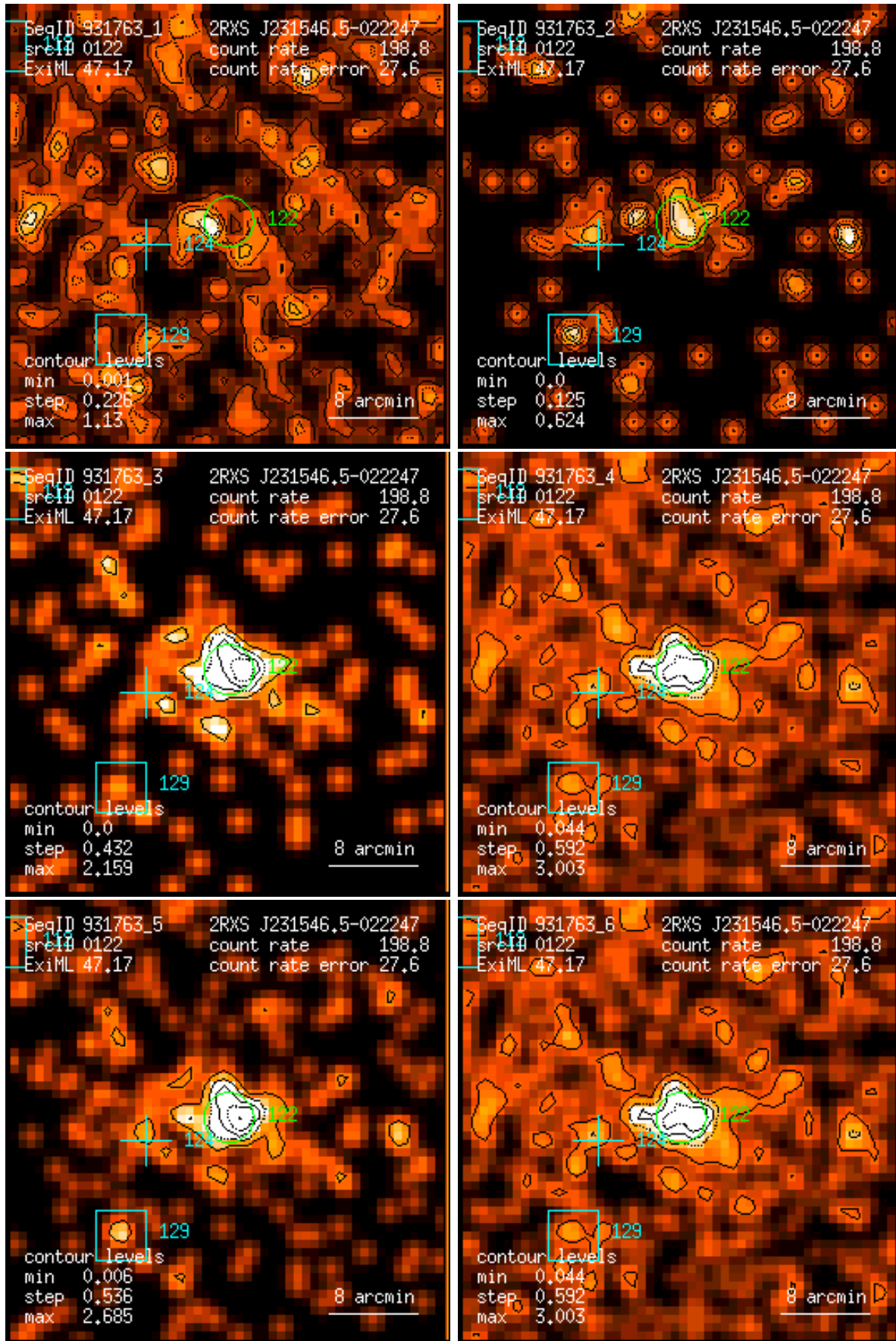
Figure 122: RASS 931763: detection 0122: band rate images, Gaussian filter: (1) PSPC channels 11 – 41, (2) 52 – 90, (3) 91 – 201, (4) 11 – 235, (5) 52 – 201, (6) 11 – 201. Broad band rates in counts/ks. Band rate contour levels in counts/ks/arcmin 2 .
