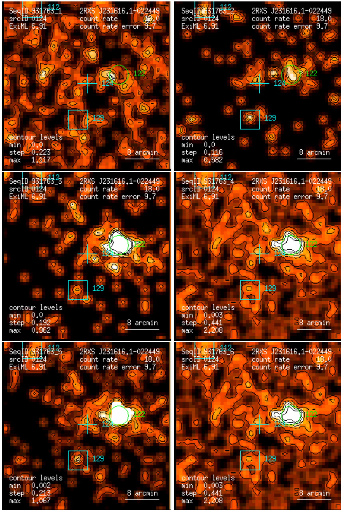
Figure 124: RASS 931763: detection 0124: band rate images, Gaussian filter: (1) PSPC channels 11 – 41, (2) 52 – 90, (3) 91 – 201, (4) 11 – 235, (5) 52 – 201, (6) 11 – 201. Broad band rates in counts/ks. Band rate contour levels in counts/ks/arcmin 2 .
