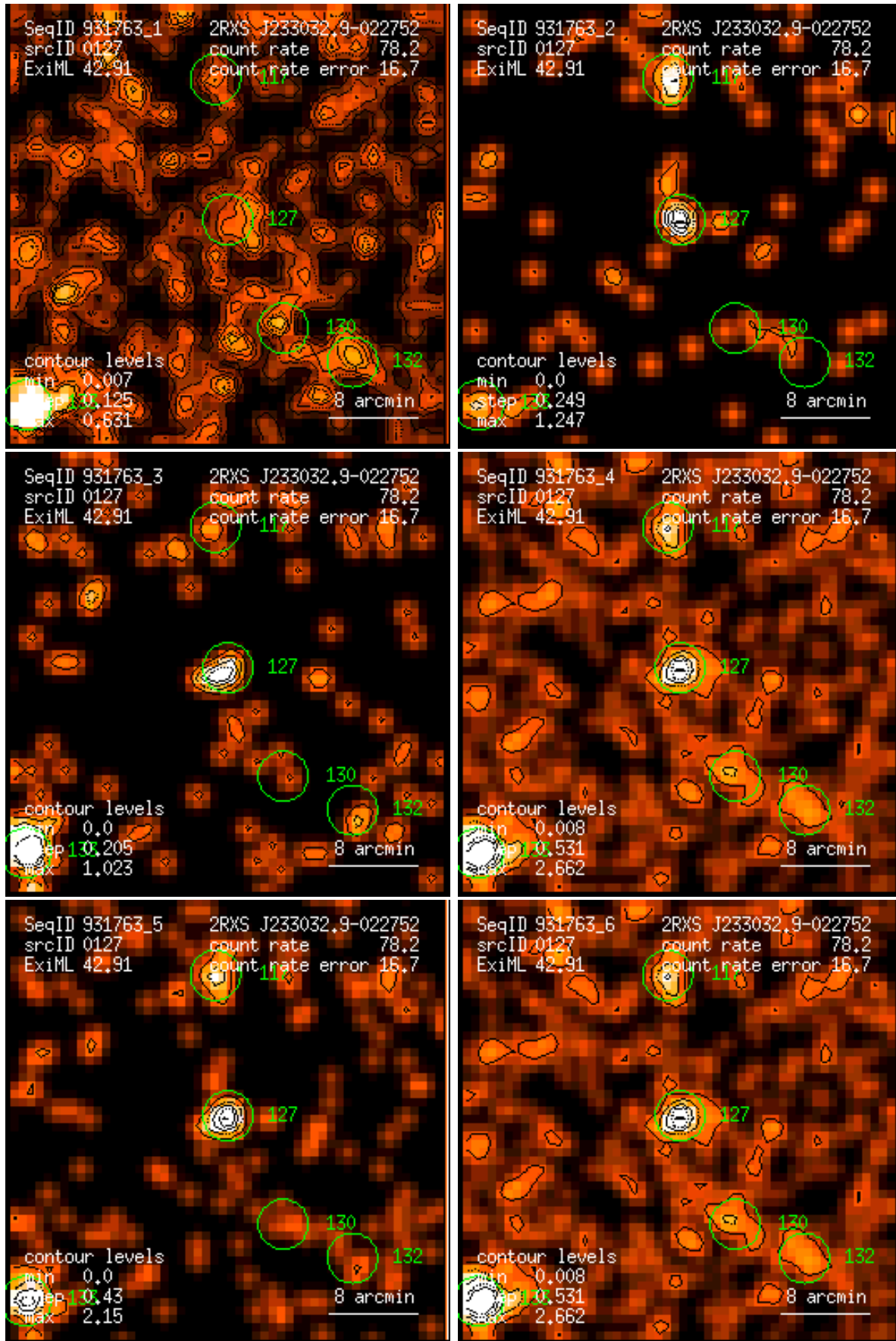
Figure 127: RASS 931763: detection 0127: band rate images, Gaussian filter: (1) PSPC channels 11 – 41, (2) 52 – 90, (3) 91 – 201, (4) 11 – 235, (5) 52 – 201, (6) 11 – 201. Broad band rates in counts/ks. Band rate contour levels in counts/ks/arcmin 2 .
