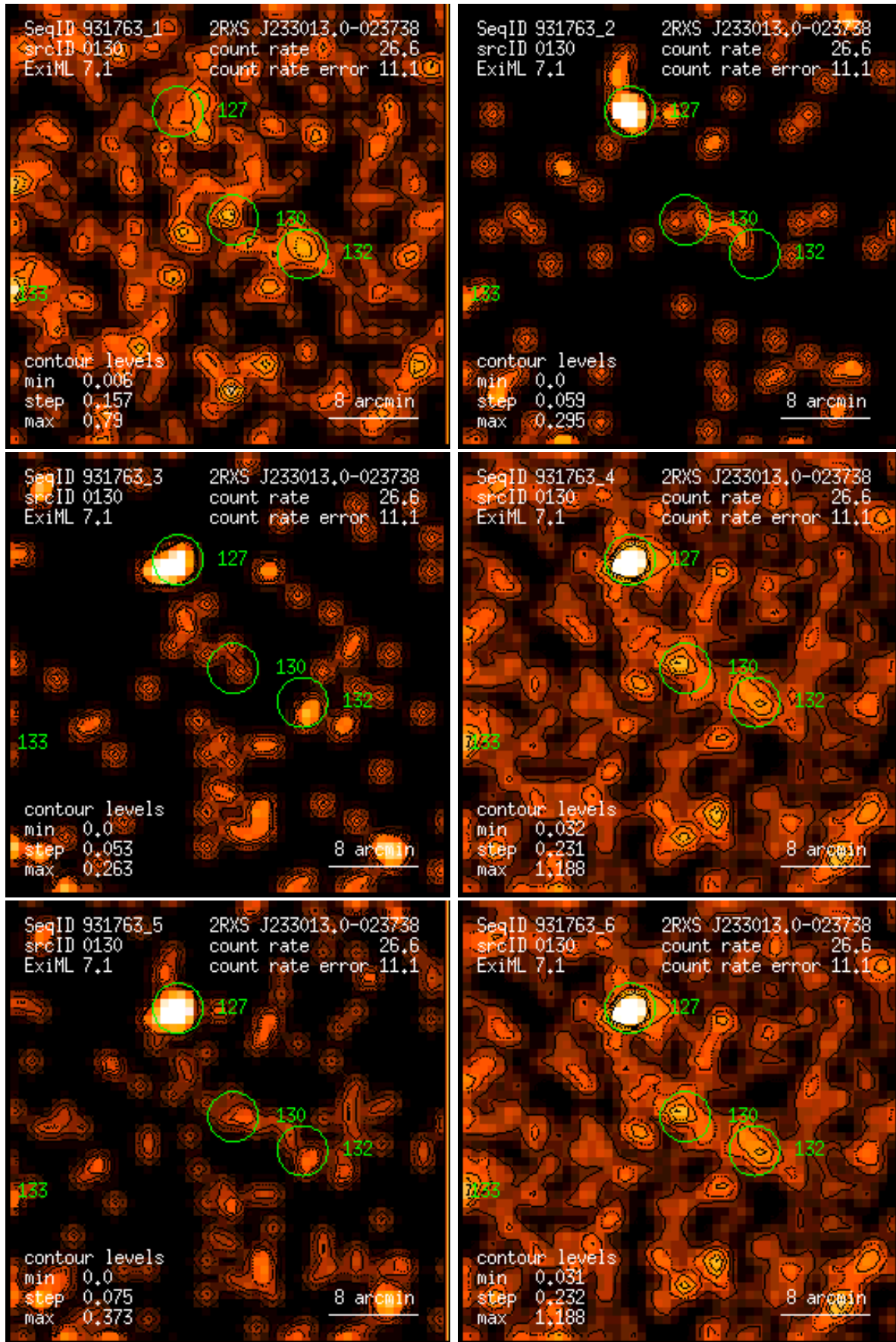
Figure 130: RASS 931763: detection 0130: band rate images, Gaussian filter: (1) PSPC channels 11 – 41, (2) 52 – 90, (3) 91 – 201, (4) 11 – 235, (5) 52 – 201, (6) 11 – 201. Broad band rates in counts/ks. Band rate contour levels in counts/ks/arcmin 2 .
