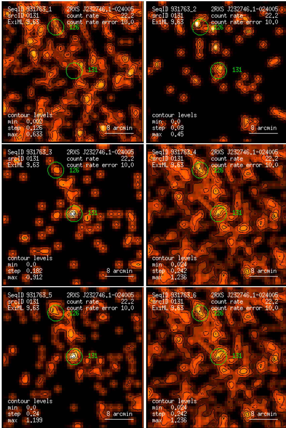
Figure 131: RASS 931763: detection 0131: band rate images, Gaussian filter: (1) PSPC channels 11 – 41, (2) 52 – 90, (3) 91 – 201, (4) 11 – 235, (5) 52 – 201, (6) 11 – 201. Broad band rates in counts/ks. Band rate contour levels in counts/ks/arcmin 2 .
