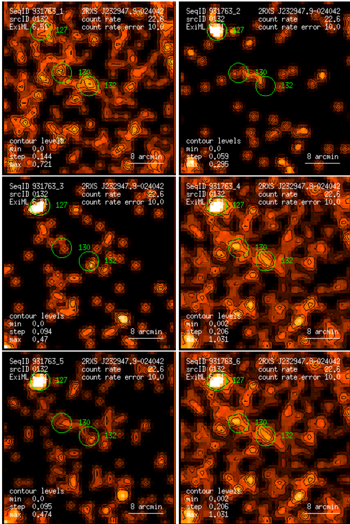
Figure 132: RASS 931763: detection 0132: band rate images, Gaussian filter: (1) PSPC channels 11 – 41, (2) 52 – 90, (3) 91 – 201, (4) 11 – 235, (5) 52 – 201, (6) 11 – 201. Broad band rates in counts/ks. Band rate contour levels in counts/ks/arcmin 2 .
