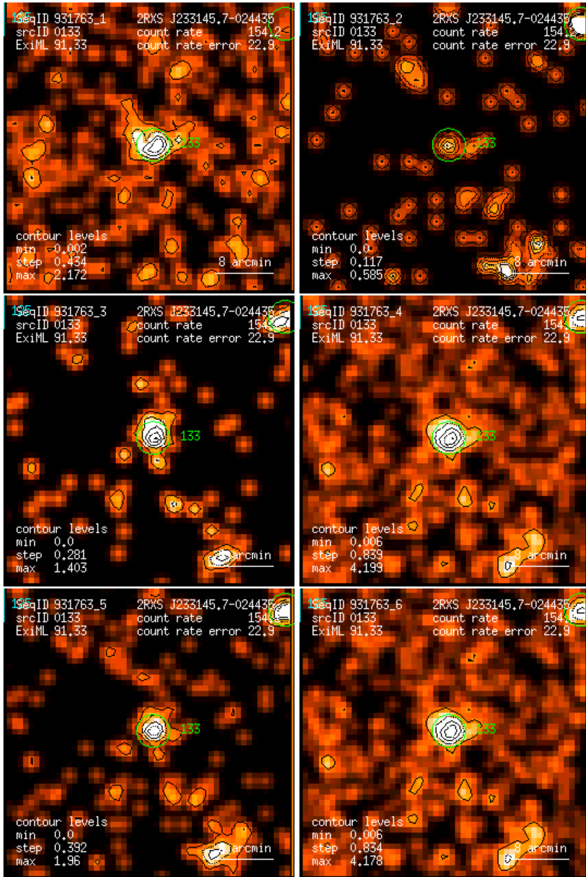
Figure 133: RASS 931763: detection 0133: band rate images, Gaussian filter: (1) PSPC channels 11 – 41, (2) 52 – 90, (3) 91 – 201, (4) 11 – 235, (5) 52 – 201, (6) 11 – 201. Broad band rates in counts/ks. Band rate contour levels in counts/ks/arcmin 2 .
