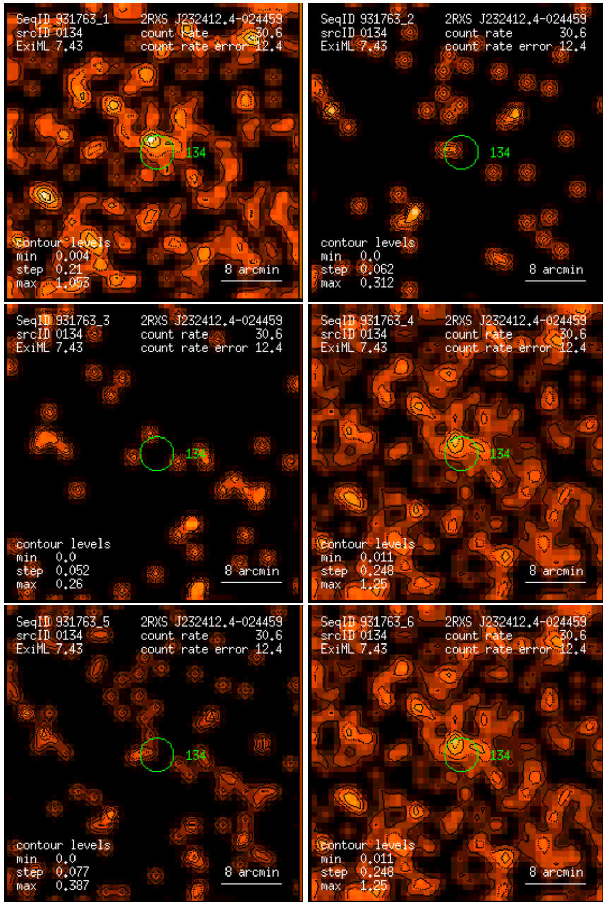
Figure 134: RASS 931763: detection 0134: band rate images, Gaussian filter: (1) PSPC channels 11 – 41, (2) 52 – 90, (3) 91 – 201, (4) 11 – 235, (5) 52 – 201, (6) 11 – 201. Broad band rates in counts/ks. Band rate contour levels in counts/ks/arcmin 2 .
