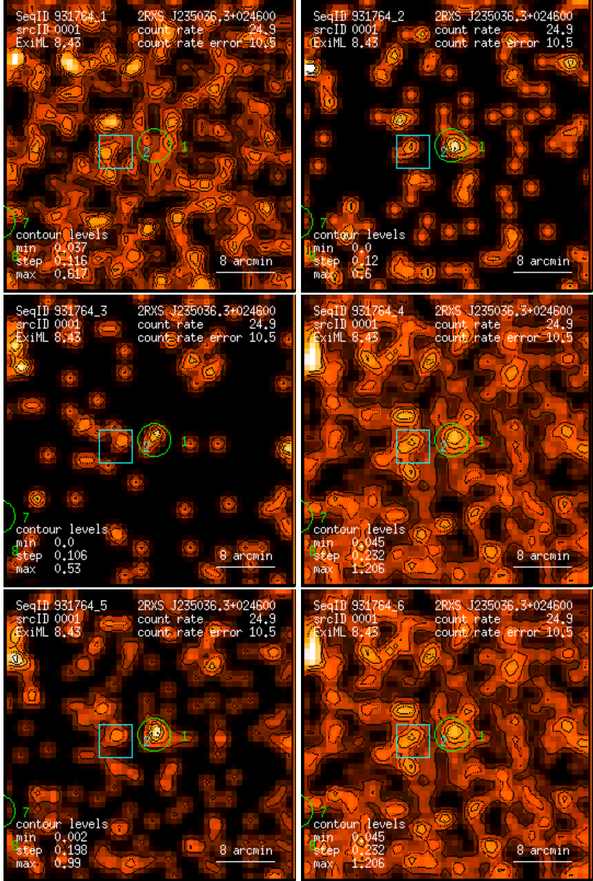
Figure 1: RASS 931764: detection 0001: band rate images, Gaussian filter: (1) PSPC channels 11 – 41, (2) 52 – 90, (3) 91 – 201, (4) 11 – 235, (5) 52 – 201, (6) 11 – 201. Broad band rates in counts/ks. Band rate contour levels in counts/ks/arcmin 2 .
