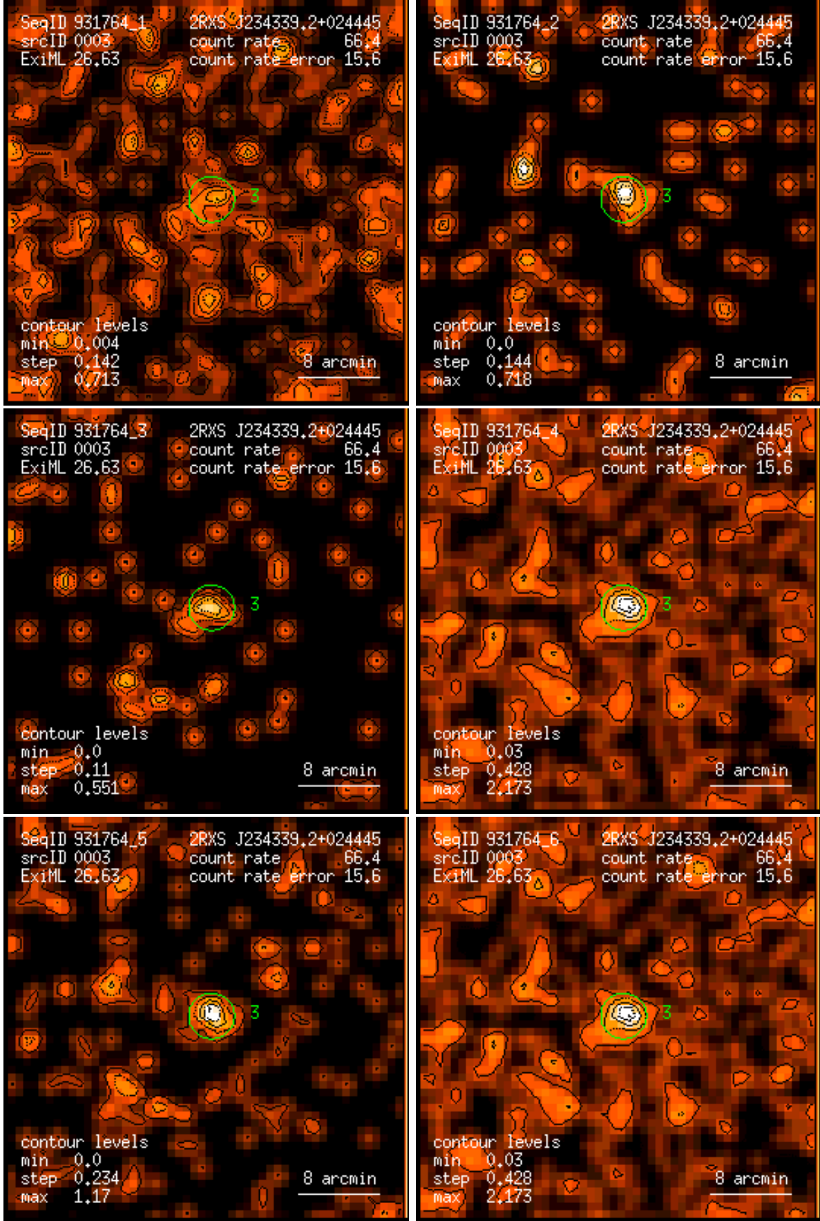
Figure 3: RASS 931764: detection 0003: band rate images, Gaussian filter: (1) PSPC channels 11 – 41, (2) 52 – 90, (3) 91 – 201, (4) 11 – 235, (5) 52 – 201, (6) 11 – 201. Broad band rates in counts/ks. Band rate contour levels in counts/ks/arcmin 2 .
