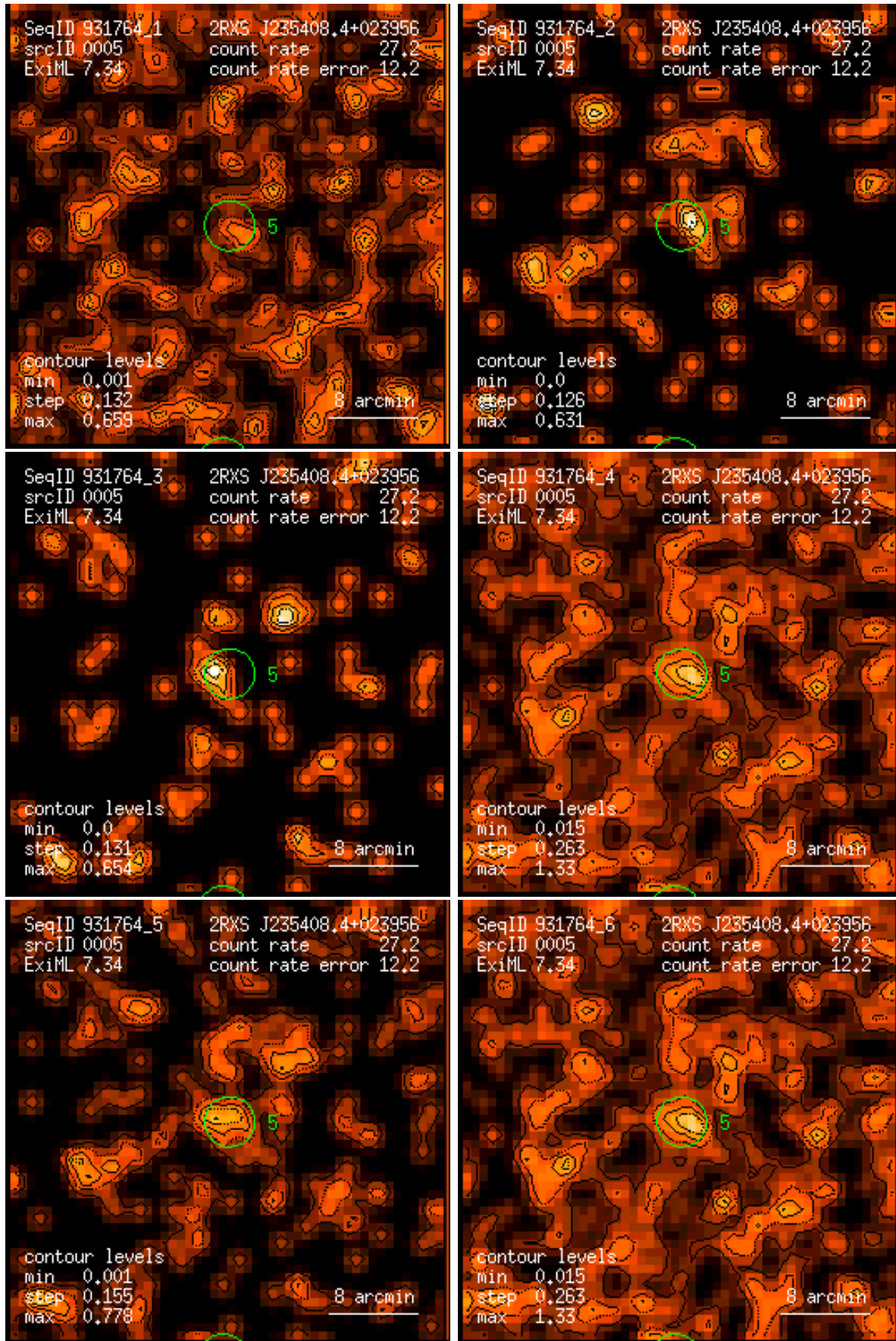
Figure 5: RASS 931764: detection 0005: band rate images, Gaussian filter: (1) PSPC channels 11 – 41, (2) 52 – 90, (3) 91 – 201, (4) 11 – 235, (5) 52 – 201, (6) 11 – 201. Broad band rates in counts/ks. Band rate contour levels in counts/ks/arcmin 2 .
