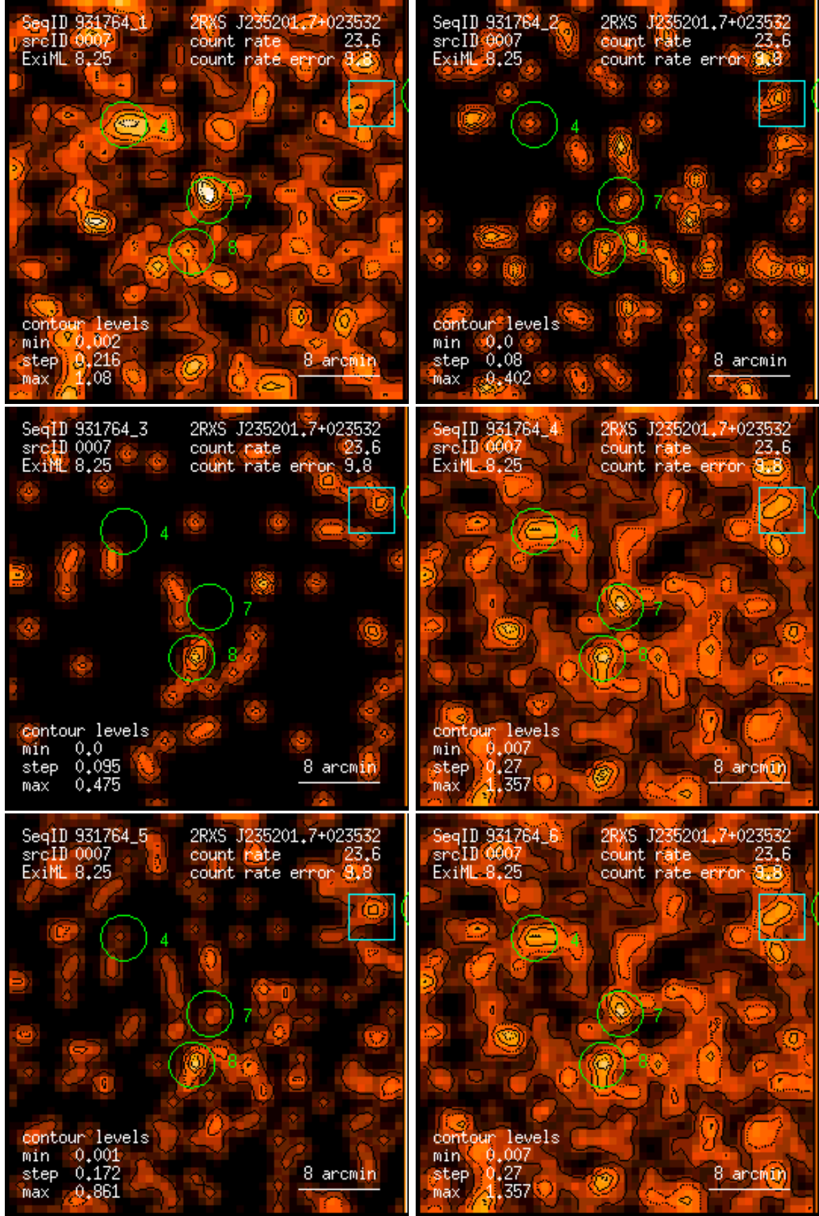
Figure 7: RASS 931764: detection 0007: band rate images, Gaussian filter: (1) PSPC channels 11 – 41, (2) 52 – 90, (3) 91 – 201, (4) 11 – 235, (5) 52 – 201, (6) 11 – 201. Broad band rates in counts/ks. Band rate contour levels in counts/ks/arcmin 2 .
