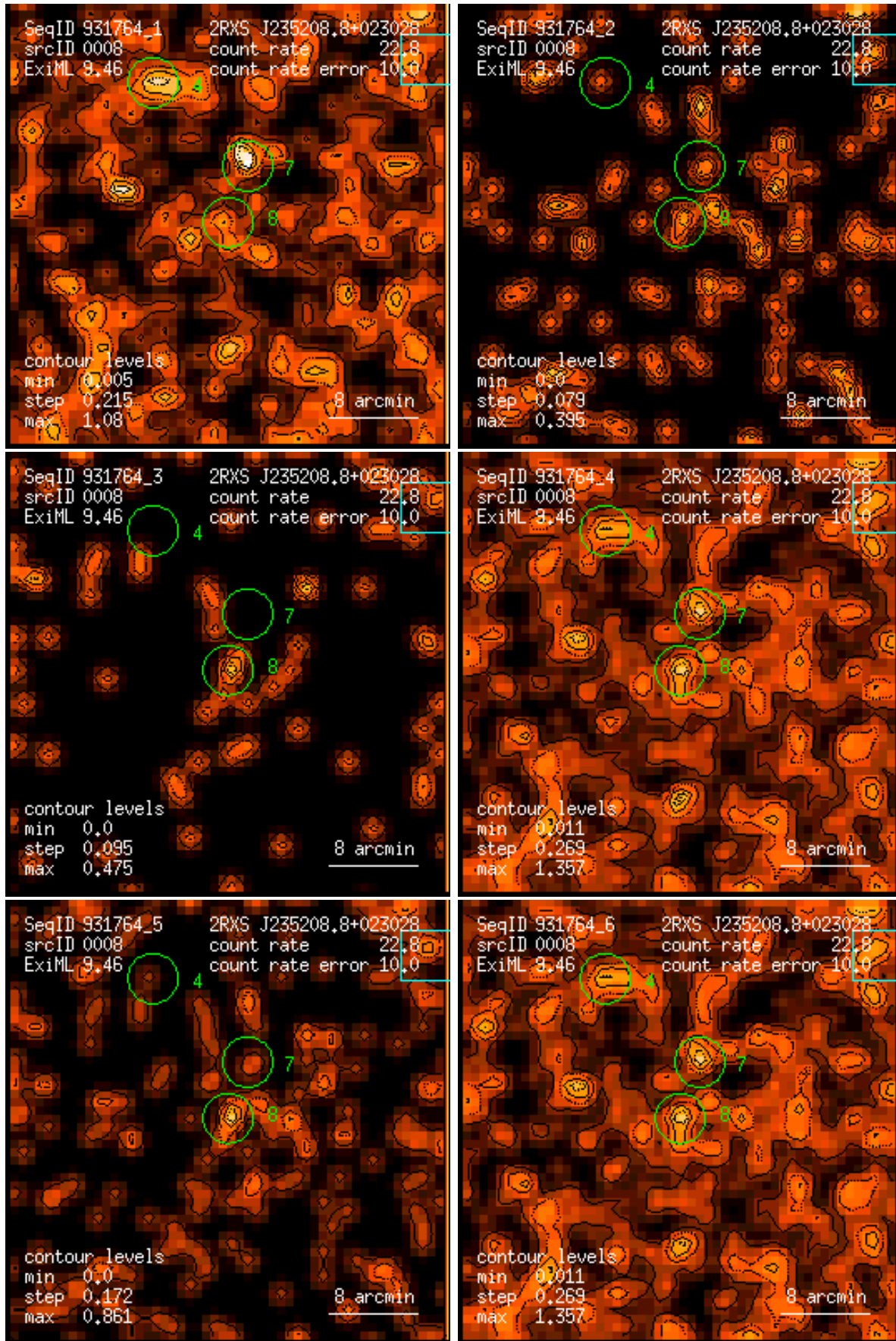
Figure 8: RASS 931764: detection 0008: band rate images, Gaussian filter: (1) PSPC channels 11 – 41, (2) 52 – 90, (3) 91 – 201, (4) 11 – 235, (5) 52 – 201, (6) 11 – 201. Broad band rates in counts/ks. Band rate contour levels in counts/ks/arcmin 2 .
