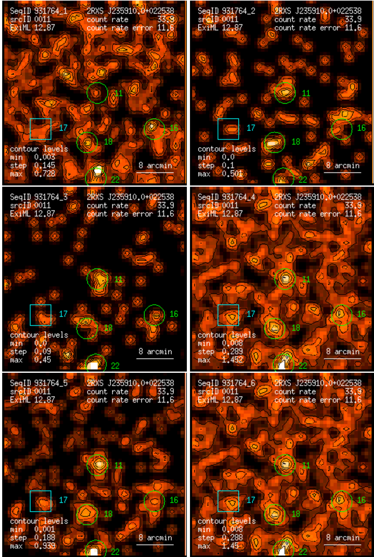
Figure 11: RASS 931764: detection 0011: band rate images, Gaussian filter: (1) PSPC channels 11 – 41, (2) 52 – 90, (3) 91 – 201, (4) 11 – 235, (5) 52 – 201, (6) 11 – 201. Broad band rates in counts/ks. Band rate contour levels in counts/ks/arcmin 2 .
