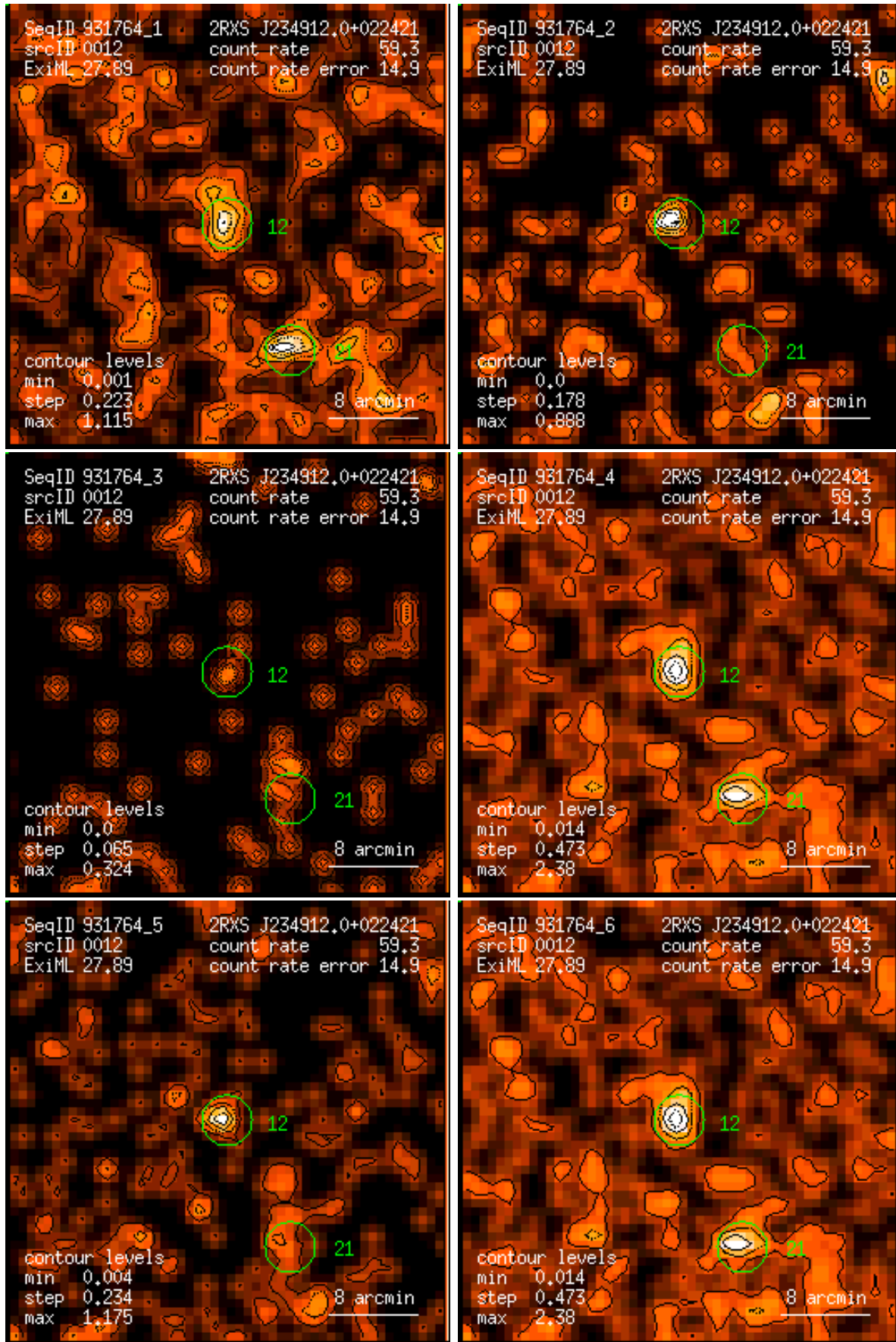
Figure 12: RASS 931764: detection 0012: band rate images, Gaussian filter: (1) PSPC channels 11 – 41, (2) 52 – 90, (3) 91 – 201, (4) 11 – 235, (5) 52 – 201, (6) 11 – 201. Broad band rates in counts/ks. Band rate contour levels in counts/ks/arcmin 2 .
