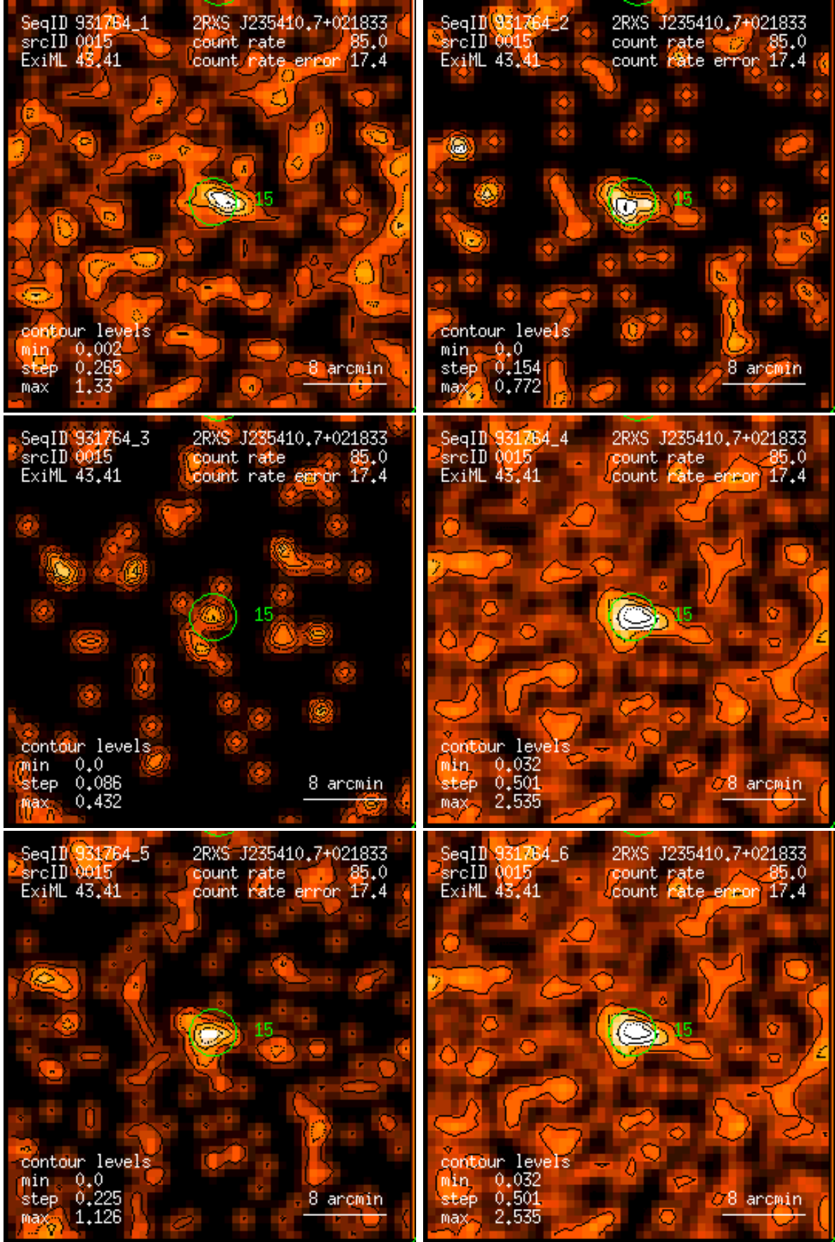
Figure 15: RASS 931764: detection 0015: band rate images, Gaussian filter: (1) PSPC channels 11 – 41, (2) 52 – 90, (3) 91 – 201, (4) 11 – 235, (5) 52 – 201, (6) 11 – 201. Broad band rates in counts/ks. Band rate contour levels in counts/ks/arcmin 2 .
