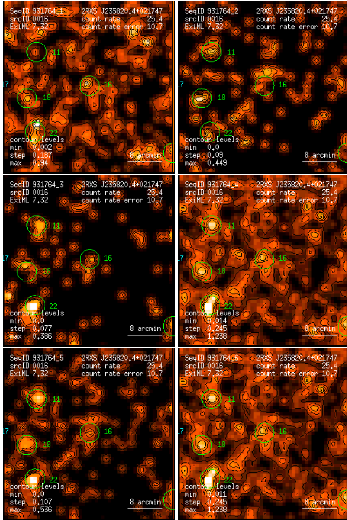
Figure 16: RASS 931764: detection 0016: band rate images, Gaussian filter: (1) PSPC channels 11 – 41, (2) 52 – 90, (3) 91 – 201, (4) 11 – 235, (5) 52 – 201, (6) 11 – 201. Broad band rates in counts/ks. Band rate contour levels in counts/ks/arcmin 2 .
