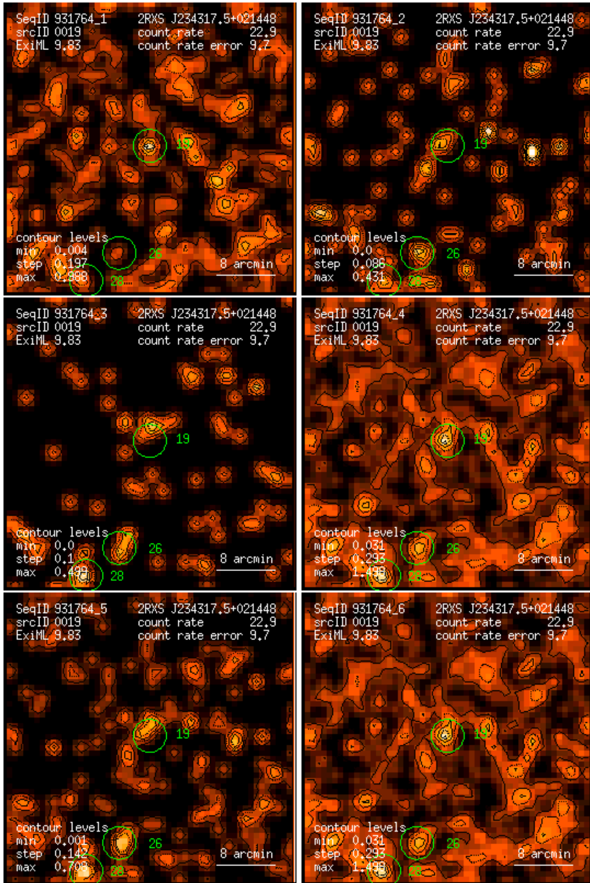
Figure 19: RASS 931764: detection 0019: band rate images, Gaussian filter: (1) PSPC channels 11 – 41, (2) 52 – 90, (3) 91 – 201, (4) 11 – 235, (5) 52 – 201, (6) 11 – 201. Broad band rates in counts/ks. Band rate contour levels in counts/ks/arcmin 2 .
