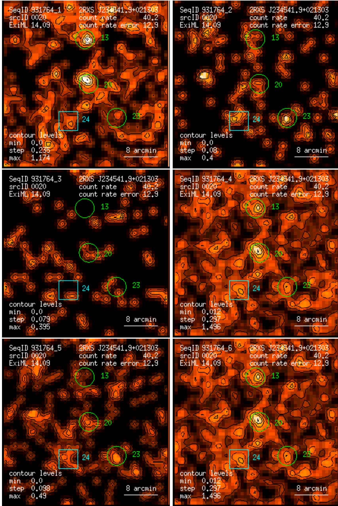
Figure 20: RASS 931764: detection 0020: band rate images, Gaussian filter: (1) PSPC channels 11 – 41, (2) 52 – 90, (3) 91 – 201, (4) 11 – 235, (5) 52 – 201, (6) 11 – 201. Broad band rates in counts/ks. Band rate contour levels in counts/ks/arcmin 2 .
