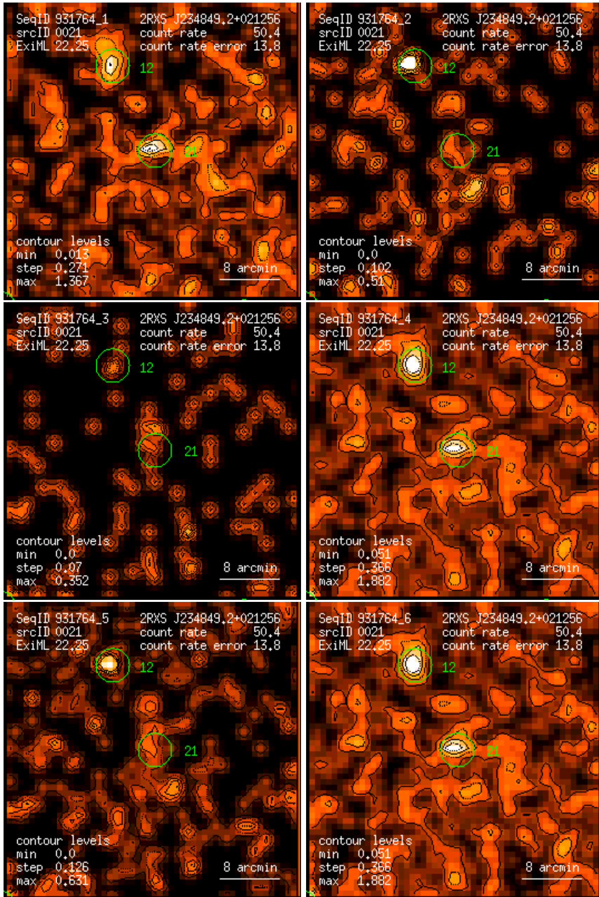
Figure 21: RASS 931764: detection 0021: band rate images, Gaussian filter: (1) PSPC channels 11 – 41, (2) 52 – 90, (3) 91 – 201, (4) 11 – 235, (5) 52 – 201, (6) 11 – 201. Broad band rates in counts/ks. Band rate contour levels in counts/ks/arcmin 2 .
