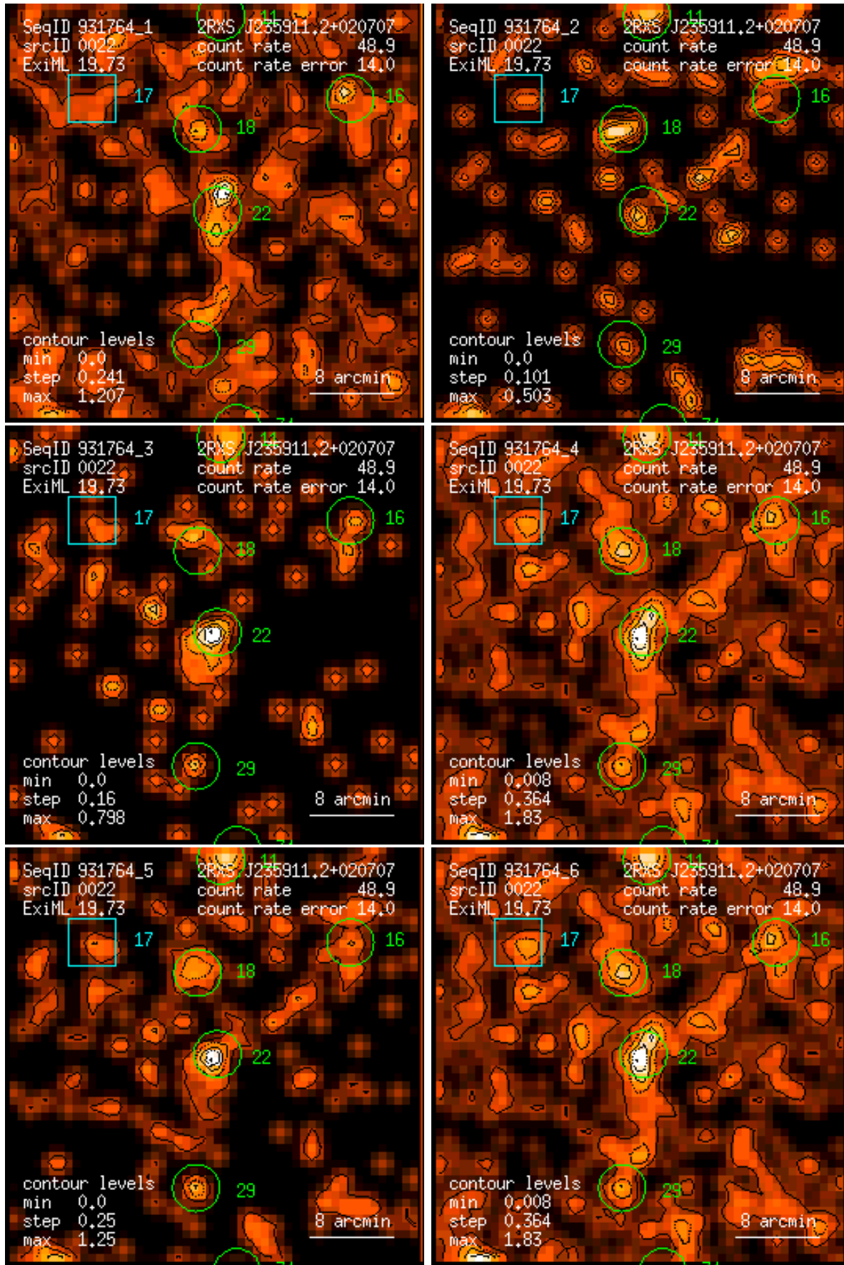
Figure 22: RASS 931764: detection 0022: band rate images, Gaussian filter: (1) PSPC channels 11 – 41, (2) 52 – 90, (3) 91 – 201, (4) 11 – 235, (5) 52 – 201, (6) 11 – 201. Broad band rates in counts/ks. Band rate contour levels in counts/ks/arcmin 2 .
