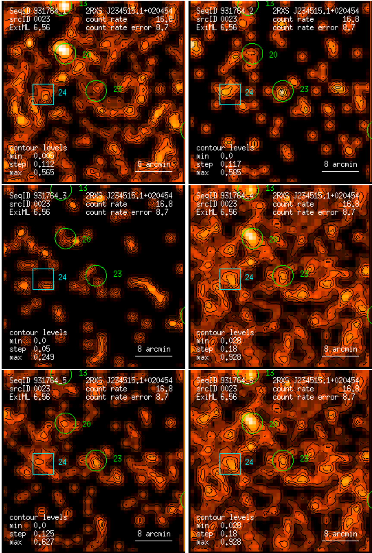
Figure 23: RASS 931764: detection 0023: band rate images, Gaussian filter: (1) PSPC channels 11 – 41, (2) 52 – 90, (3) 91 – 201, (4) 11 – 235, (5) 52 – 201, (6) 11 – 201. Broad band rates in counts/ks. Band rate contour levels in counts/ks/arcmin 2 .
