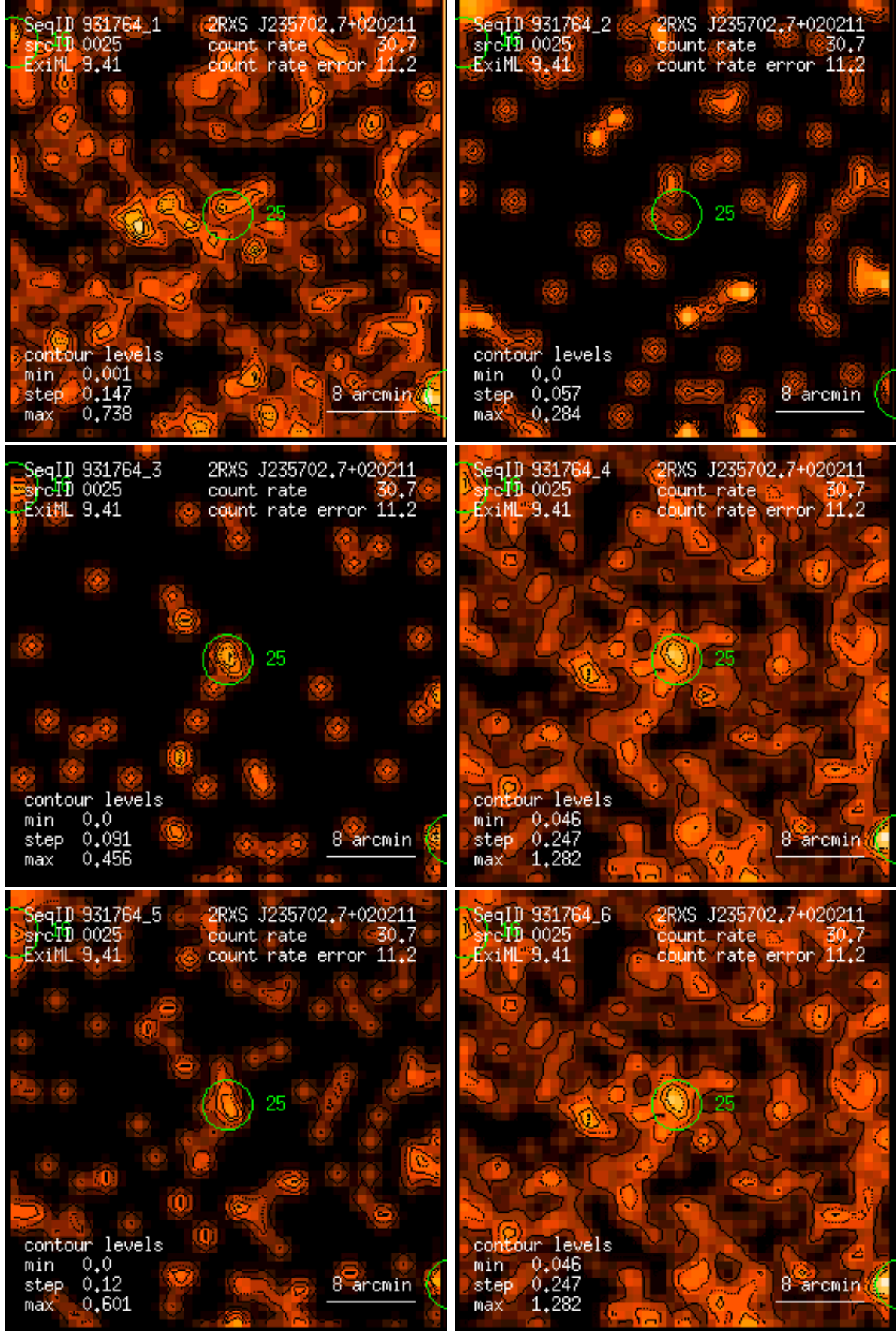
Figure 25: RASS 931764: detection 0025: band rate images, Gaussian filter: (1) PSPC channels 11 – 41, (2) 52 – 90, (3) 91 – 201, (4) 11 – 235, (5) 52 – 201, (6) 11 – 201. Broad band rates in counts/ks. Band rate contour levels in counts/ks/arcmin 2 .
