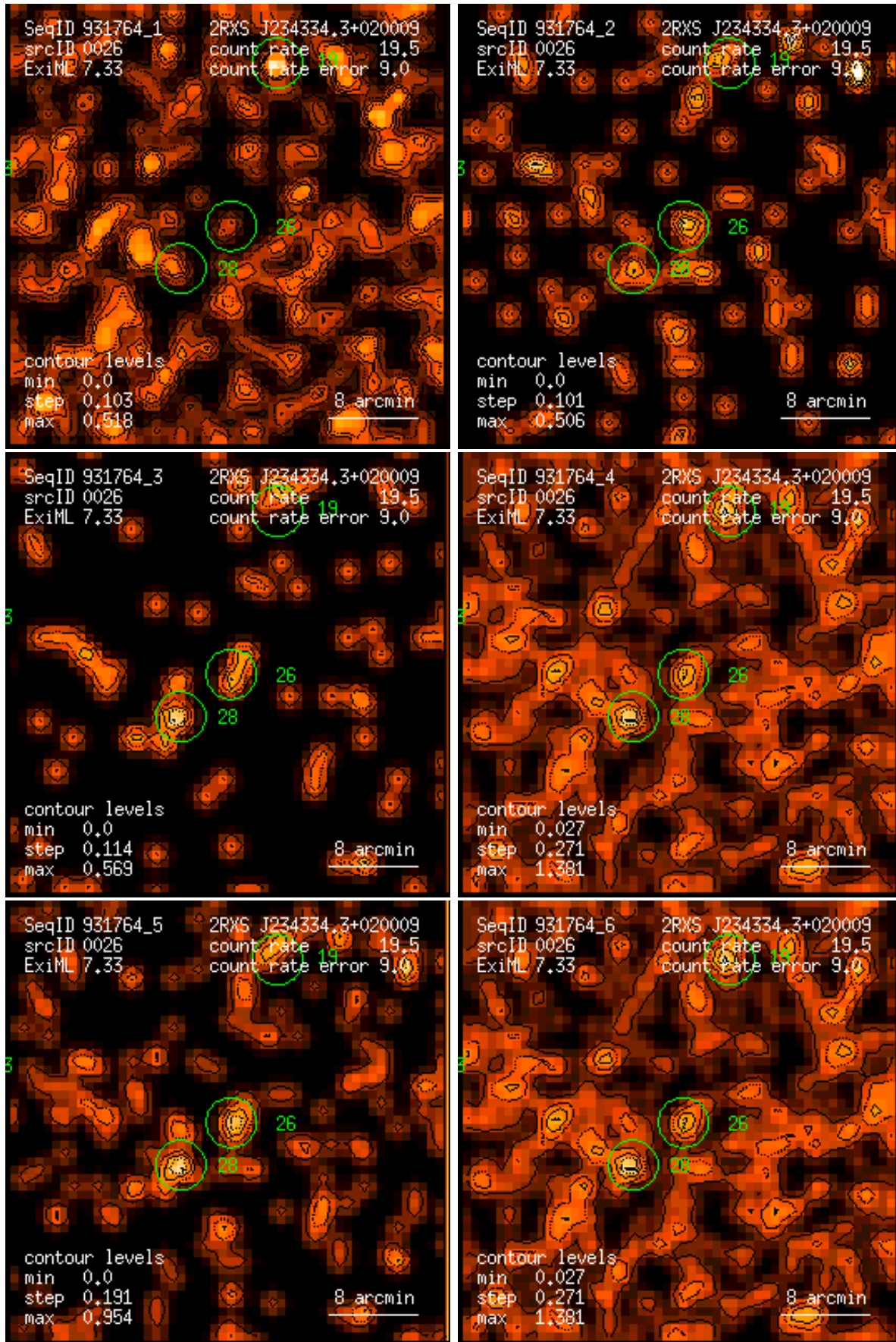
Figure 26: RASS 931764: detection 0026: band rate images, Gaussian filter: (1) PSPC channels 11 – 41, (2) 52 – 90, (3) 91 – 201, (4) 11 – 235, (5) 52 – 201, (6) 11 – 201. Broad band rates in counts/ks. Band rate contour levels in counts/ks/arcmin 2 .
