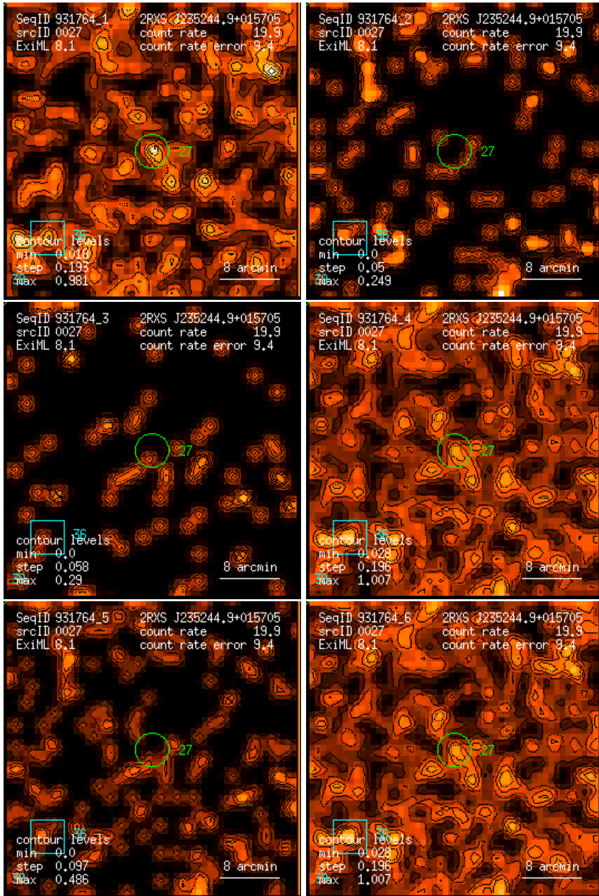
Figure 27: RASS 931764: detection 0027: band rate images, Gaussian filter: (1) PSPC channels 11 – 41, (2) 52 – 90, (3) 91 – 201, (4) 11 – 235, (5) 52 – 201, (6) 11 – 201. Broad band rates in counts/ks. Band rate contour levels in counts/ks/arcmin 2 .
