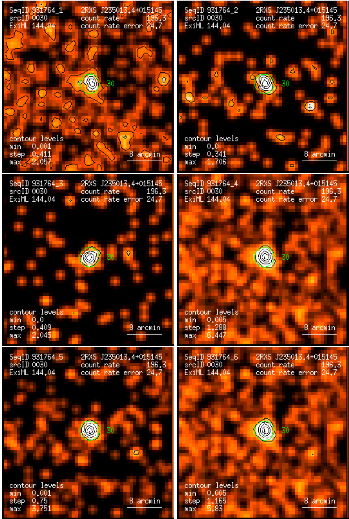
Figure 30: RASS 931764: detection 0030: band rate images, Gaussian filter: (1) PSPC channels 11 – 41, (2) 52 – 90, (3) 91 – 201, (4) 11 – 235, (5) 52 – 201, (6) 11 – 201. Broad band rates in counts/ks. Band rate contour levels in counts/ks/arcmin 2 .
