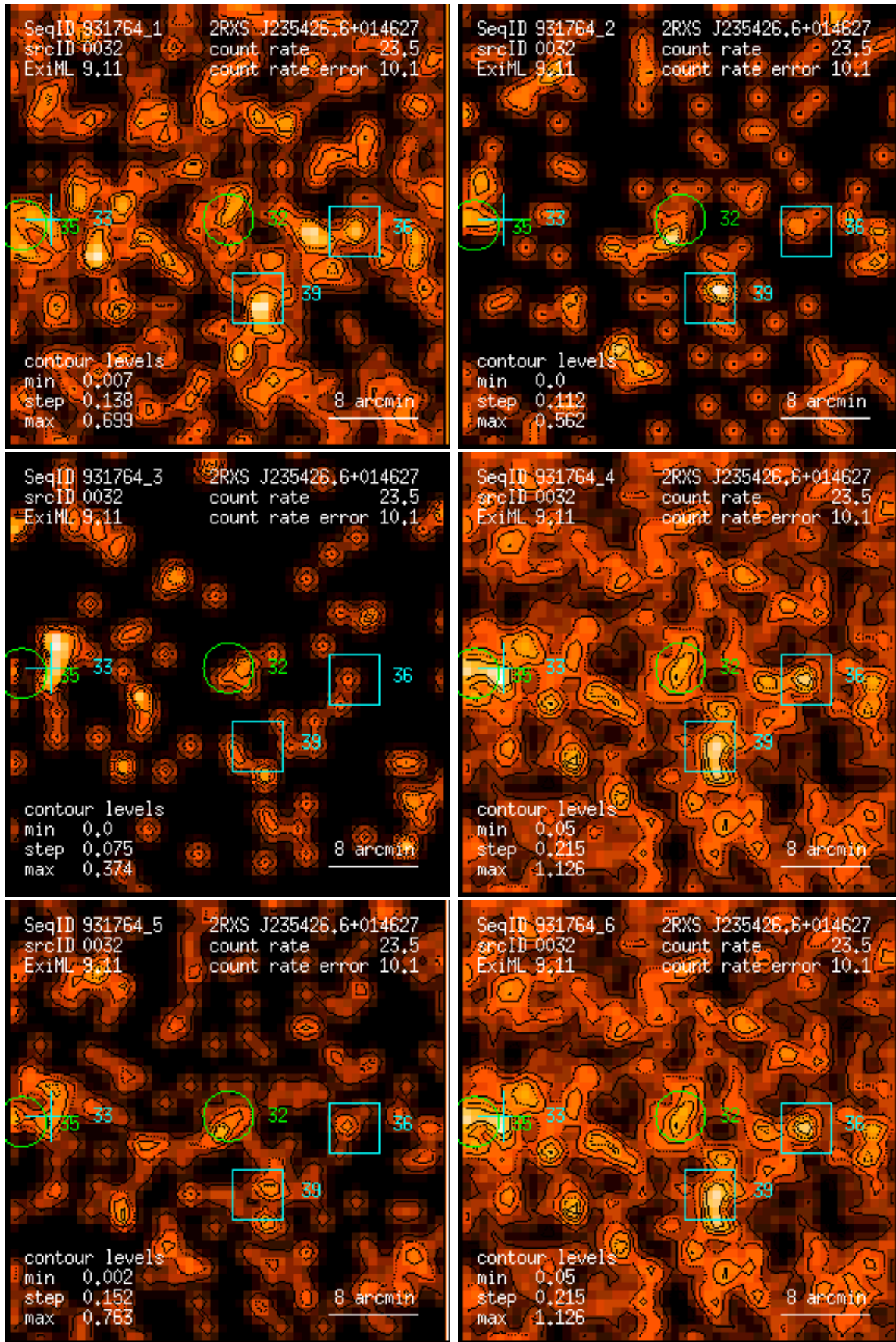
Figure 32: RASS 931764: detection 0032: band rate images, Gaussian filter: (1) PSPC channels 11 – 41, (2) 52 – 90, (3) 91 – 201, (4) 11 – 235, (5) 52 – 201, (6) 11 – 201. Broad band rates in counts/ks. Band rate contour levels in counts/ks/arcmin 2 .
