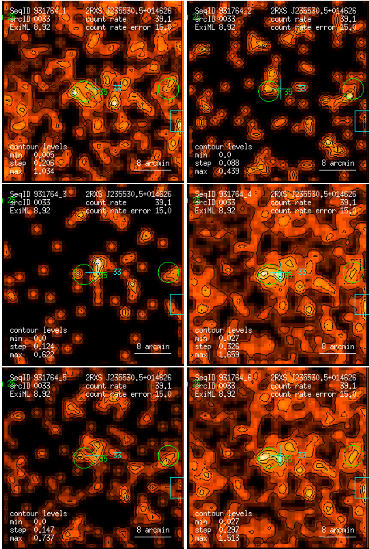
Figure 33: RASS 931764: detection 0033: band rate images, Gaussian filter: (1) PSPC channels 11 – 41, (2) 52 – 90, (3) 91 – 201, (4) 11 – 235, (5) 52 – 201, (6) 11 – 201. Broad band rates in counts/ks. Band rate contour levels in counts/ks/arcmin 2 .
