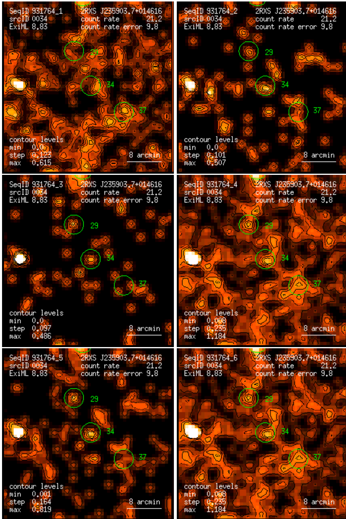
Figure 34: RASS 931764: detection 0034: band rate images, Gaussian filter: (1) PSPC channels 11 – 41, (2) 52 – 90, (3) 91 – 201, (4) 11 – 235, (5) 52 – 201, (6) 11 – 201. Broad band rates in counts/ks. Band rate contour levels in counts/ks/arcmin 2 .
