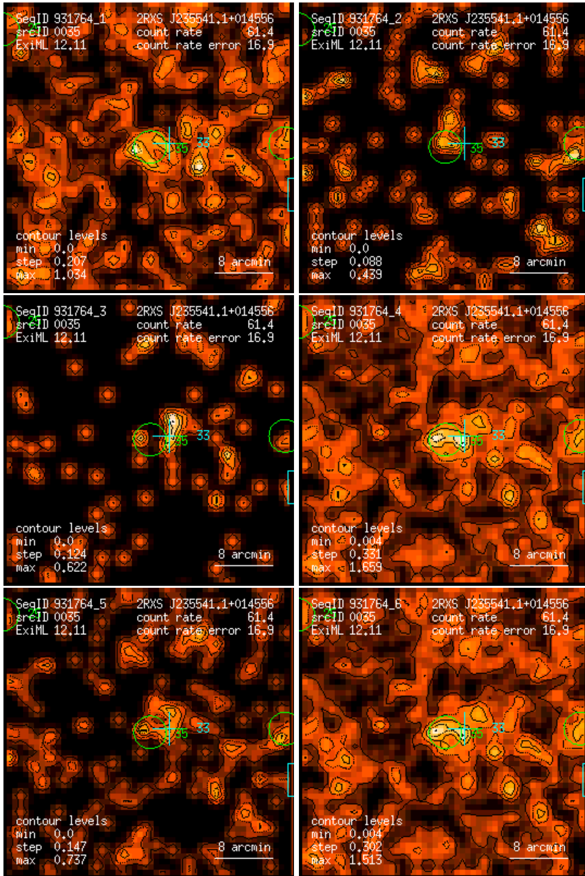
Figure 35: RASS 931764: detection 0035: band rate images, Gaussian filter: (1) PSPC channels 11 – 41, (2) 52 – 90, (3) 91 – 201, (4) 11 – 235, (5) 52 – 201, (6) 11 – 201. Broad band rates in counts/ks. Band rate contour levels in counts/ks/arcmin 2 .
