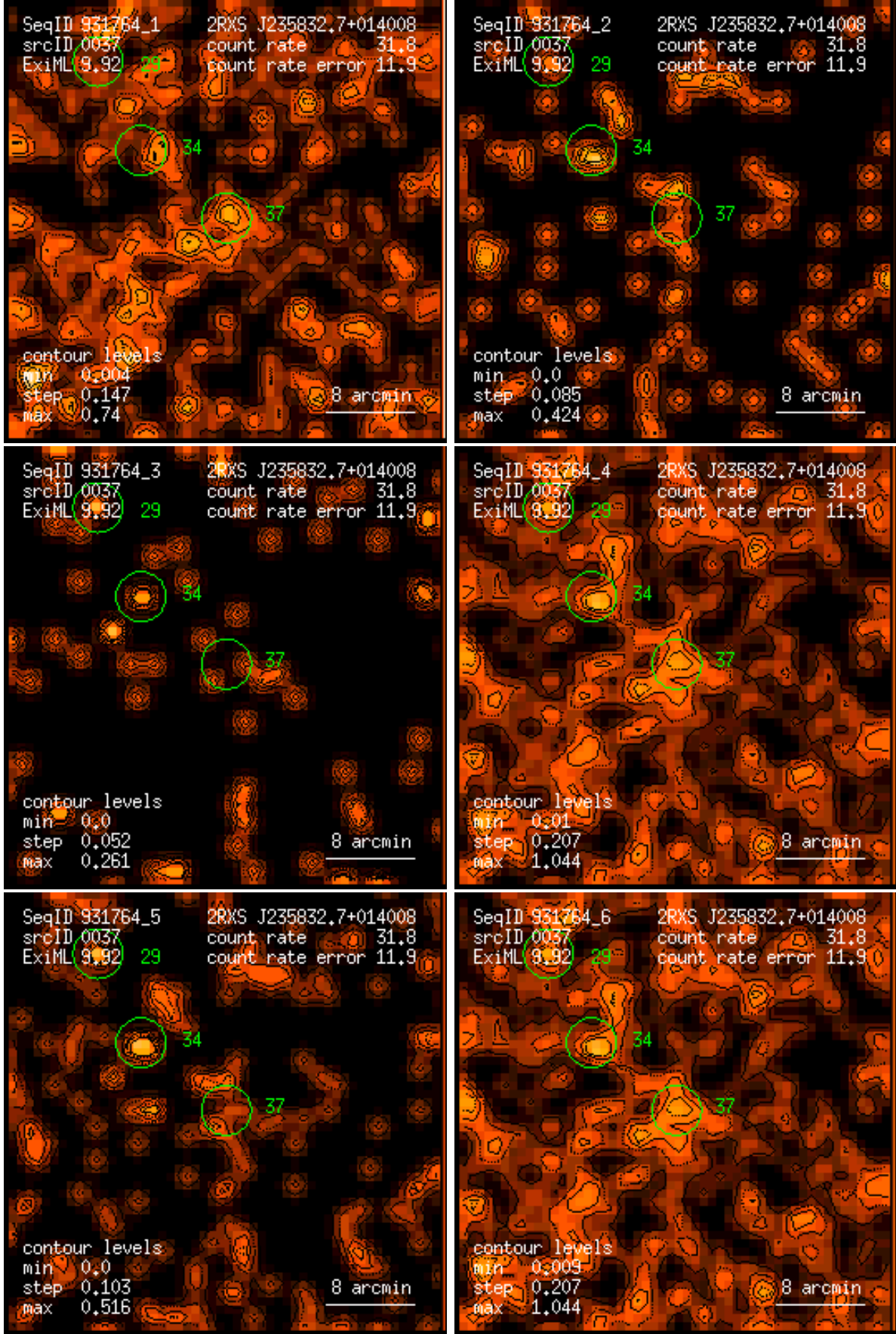
Figure 37: RASS 931764: detection 0037: band rate images, Gaussian filter: (1) PSPC channels 11 – 41, (2) 52 – 90, (3) 91 – 201, (4) 11 – 235, (5) 52 – 201, (6) 11 – 201. Broad band rates in counts/ks. Band rate contour levels in counts/ks/arcmin 2 .
