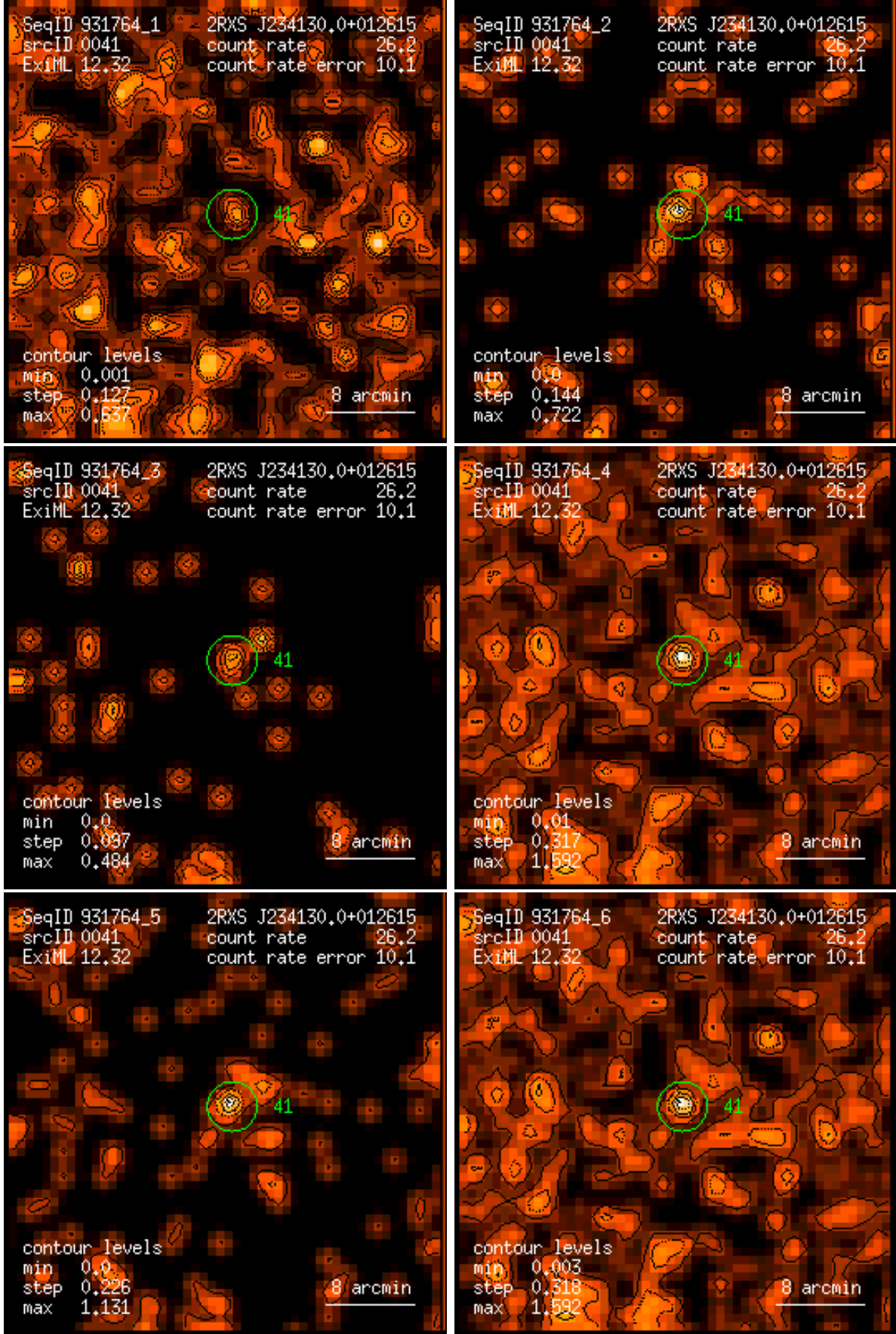
Figure 41: RASS 931764: detection 0041: band rate images, Gaussian filter: (1) PSPC channels 11 – 41, (2) 52 – 90, (3) 91 – 201, (4) 11 – 235, (5) 52 – 201, (6) 11 – 201. Broad band rates in counts/ks. Band rate contour levels in counts/ks/arcmin 2 .
